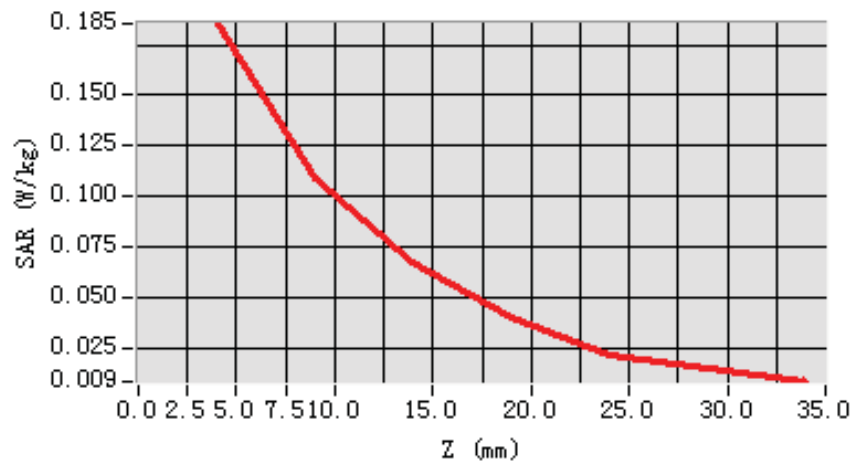
SAR, Z Axis Scan (X = 8, Y = -41)
