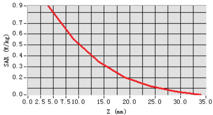
SAR, Z Axis Scan (X = -50, Y = -32)
