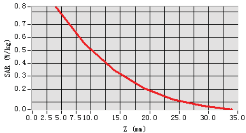
SAR, Z Axis Scan (X = -51, Y = -32)
