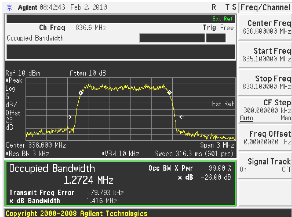
(Plot H: CDMA 800-EVDO Channel = 384)
