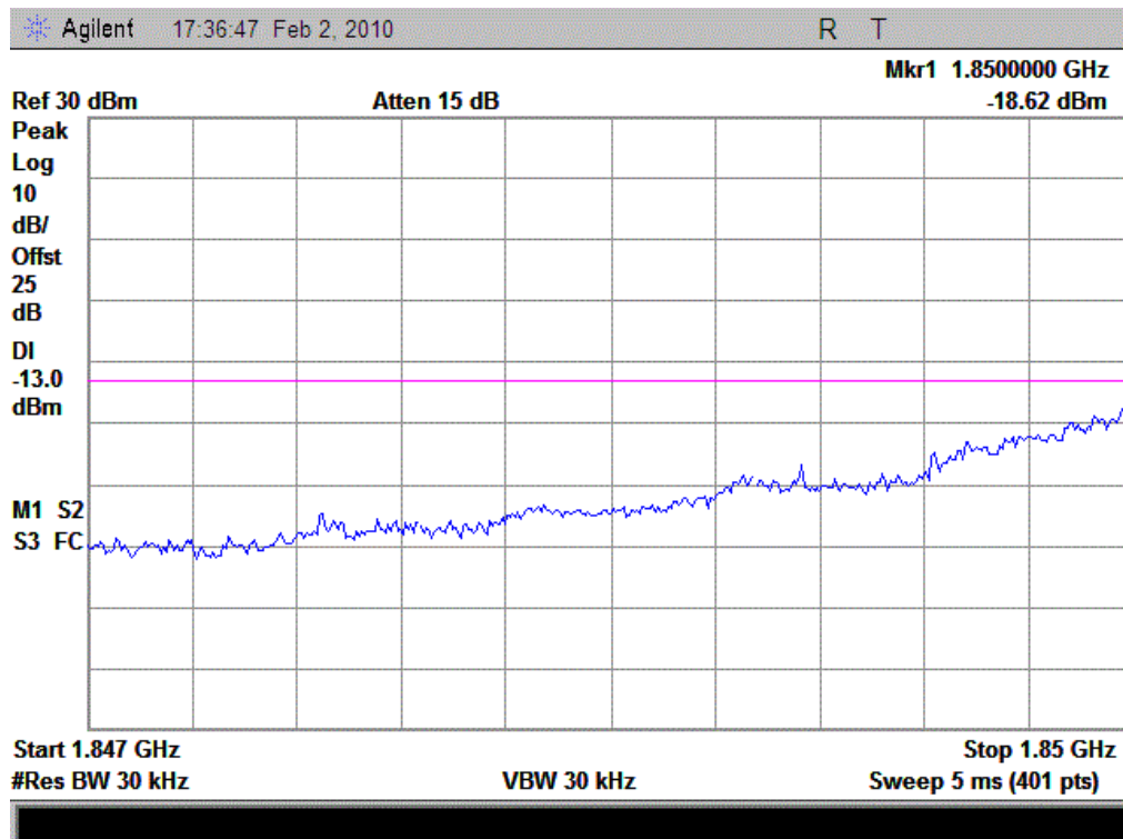
(Plot G: CDMA 1900-EVDO Channel = 25)
