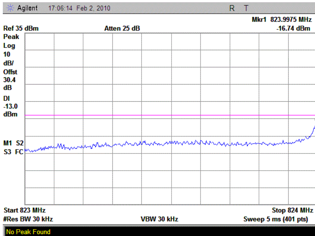
(Plot E: CDMA 800-EVDO Channel = 1013)
