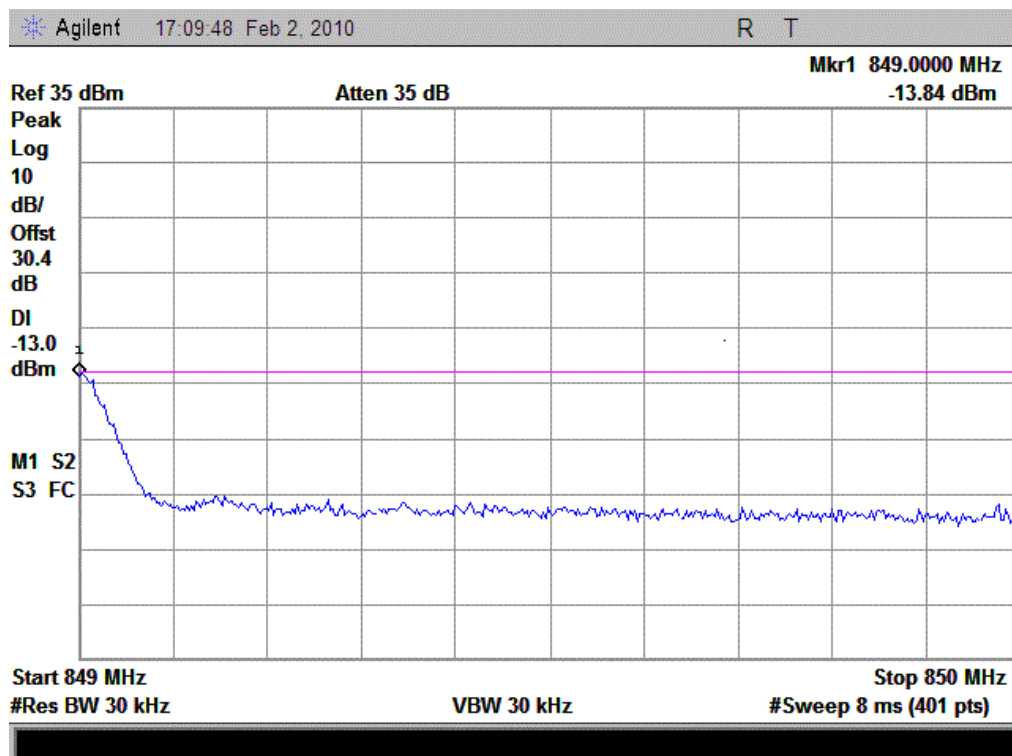
(Plot F: CDMA 800-EVDO Channel = 777)
