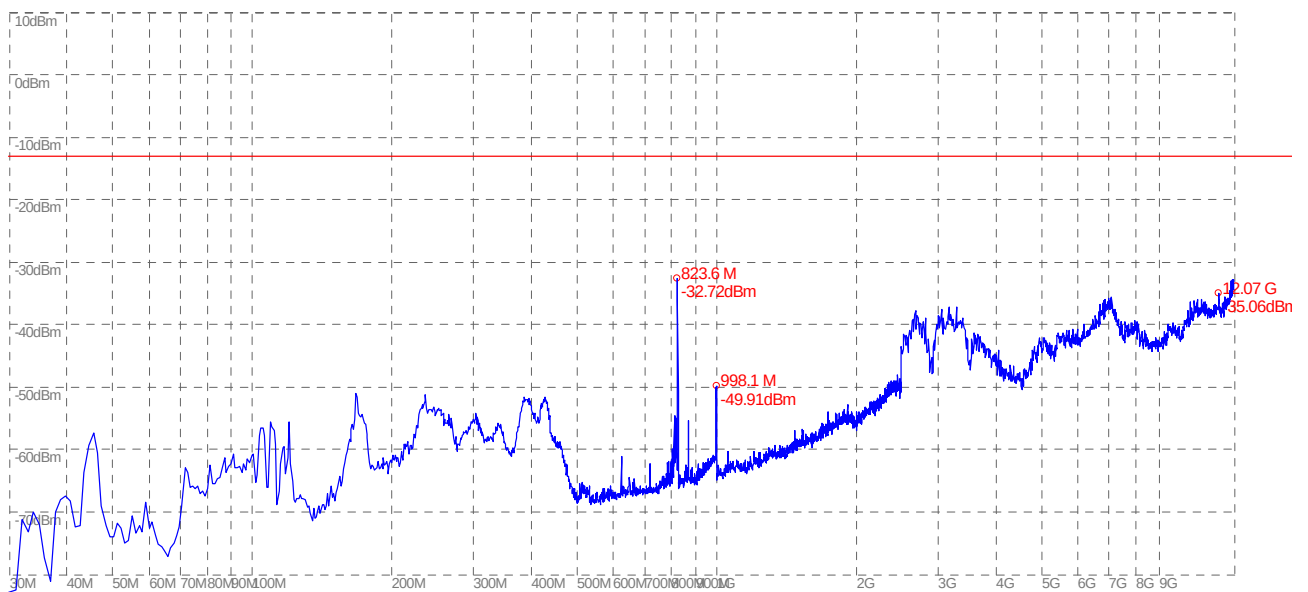
(Plot G.1: CDMA 800-EVDO Channel = 1013, Test Antenna Horizontal)
