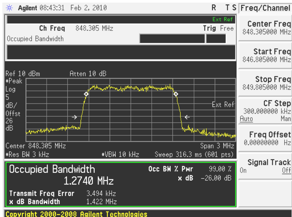
(Plot I: CDMA 800-EVDO Channel = 777)
