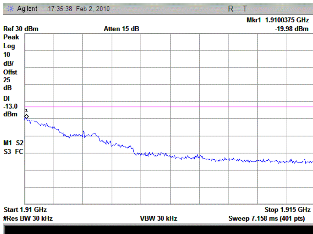
(Plot H: CDMA 1900-EVDO Channel = 1175)
