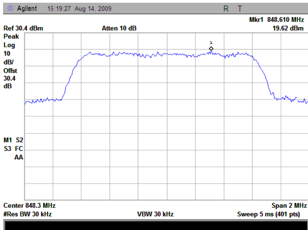
(Plot B: EVDO Channel = 777)
