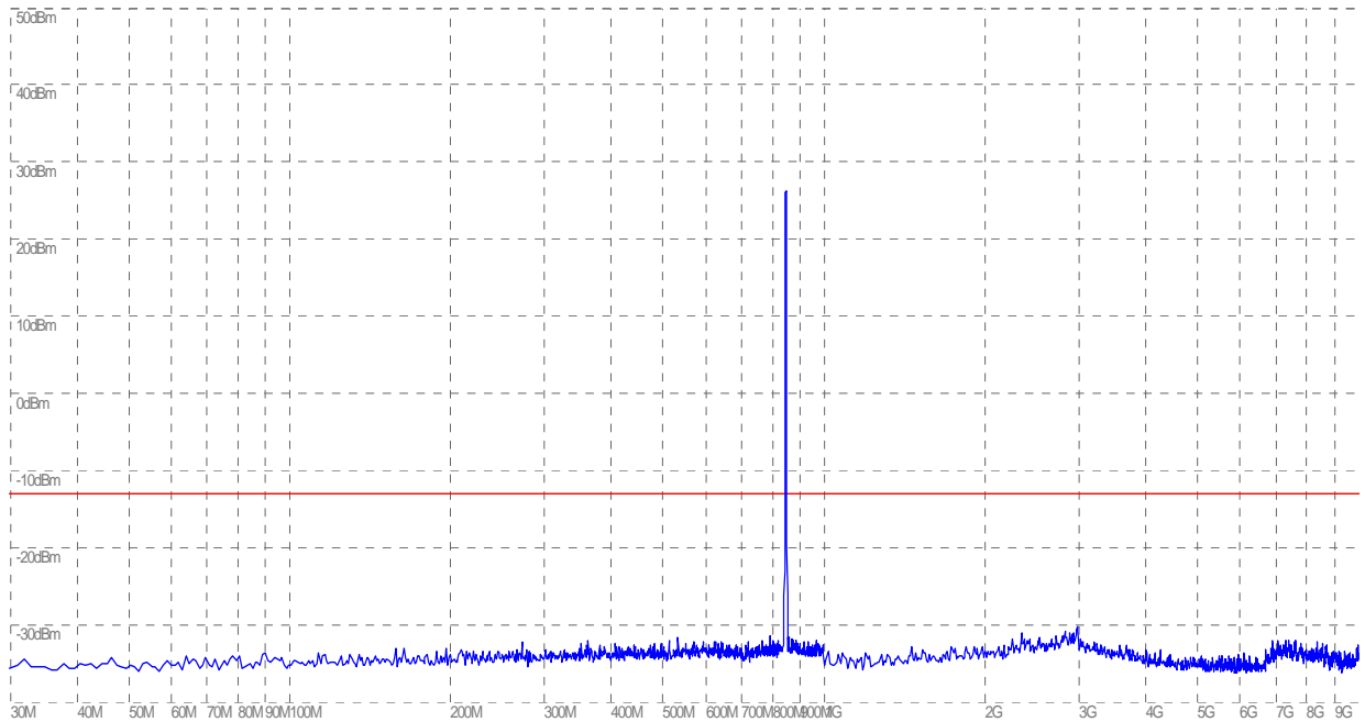
(Plot C: CDMA 800MHz Channel = 777, 30MHz to 10GHz)
