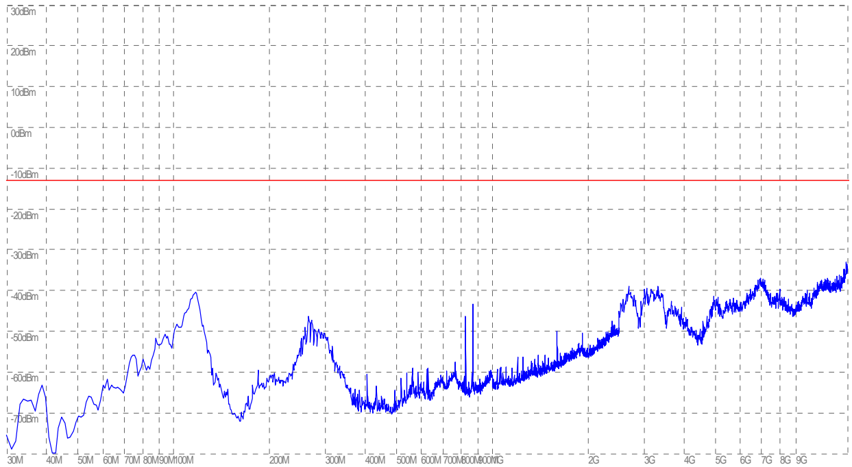
(Plot D.1: EVDO Channel = 1013, Test Antenna Horizontal)
