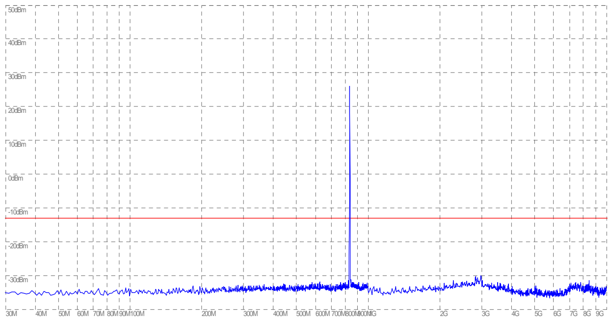
(Plot B: CDMA 800MHz Channel = 384, 30MHz to 10GHz)
