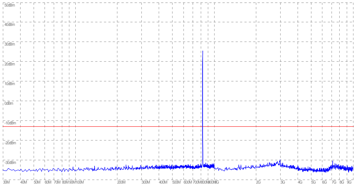
(Plot A: CDMA 800MHz Channel = 1013, 30MHz to 10GHz)
