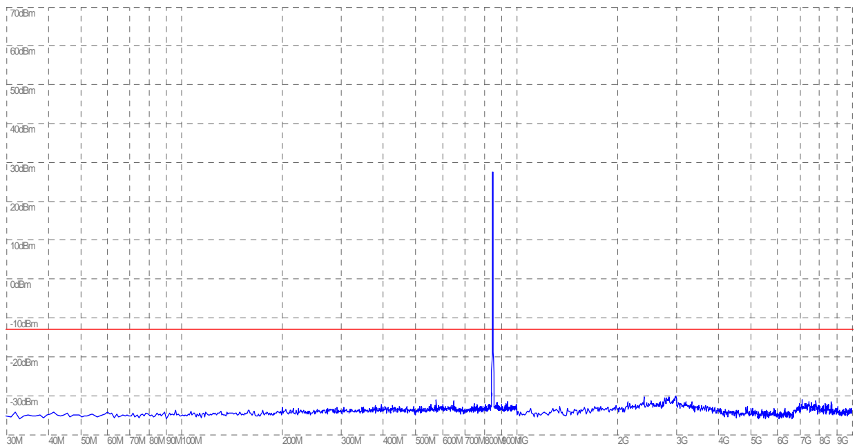
(Plot F: EVDO Channel =777, 30MHz to 10GHz)
