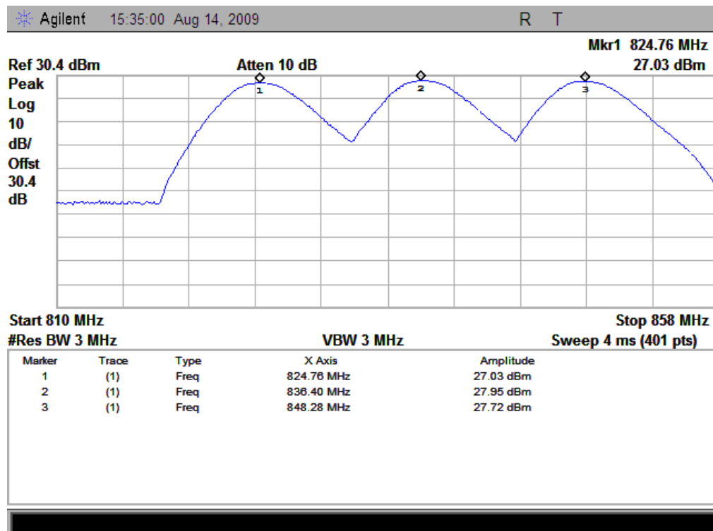
(Plot B: EVDO-FETAP Channel = 1013, 384, 777)
