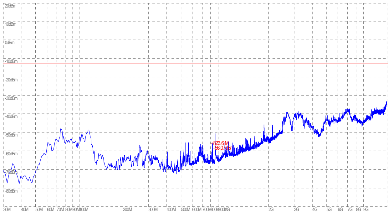
(Plot A.2: CDMA 800MHz Channel = 1013, Test Antenna Vertical)
