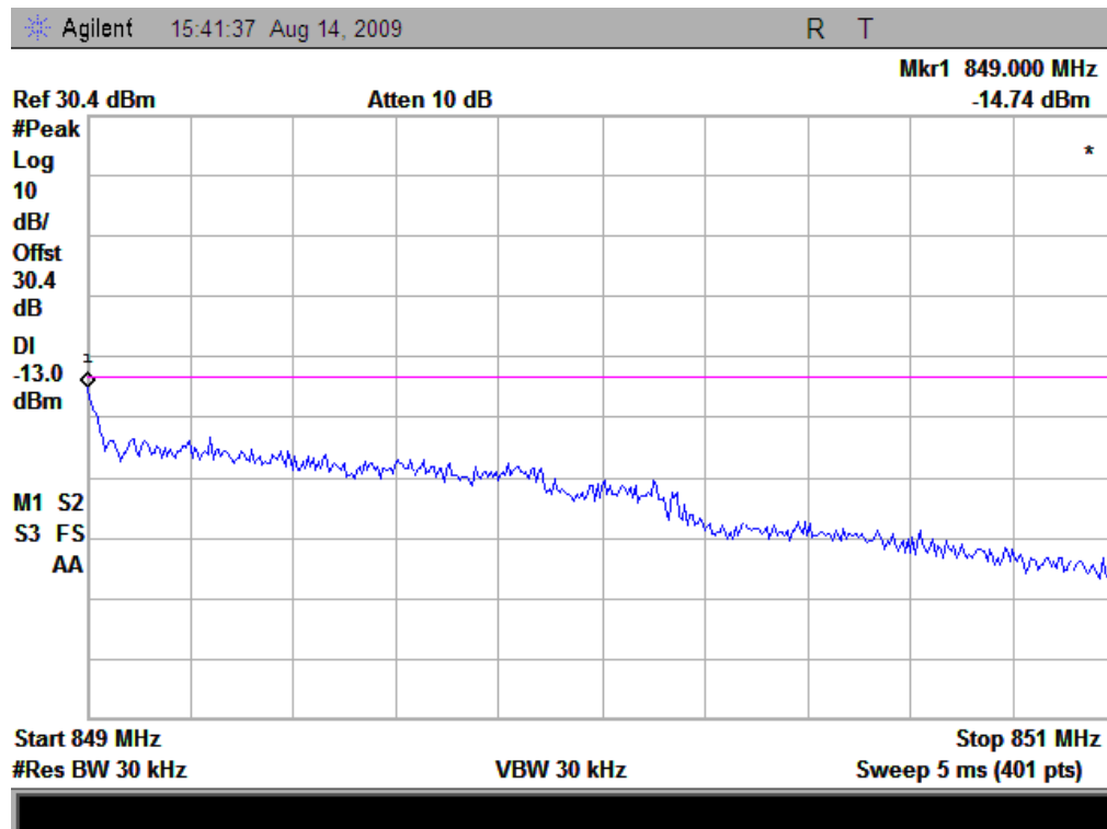
(Plot D: EVDO Channel = 777)
