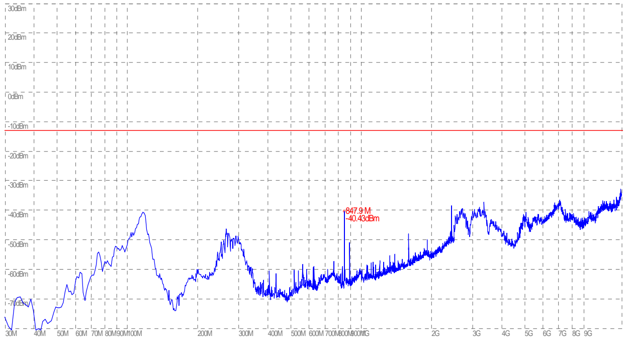
(Plot F.1: EVDO Channel = 777, Test Antenna Horizontal)
