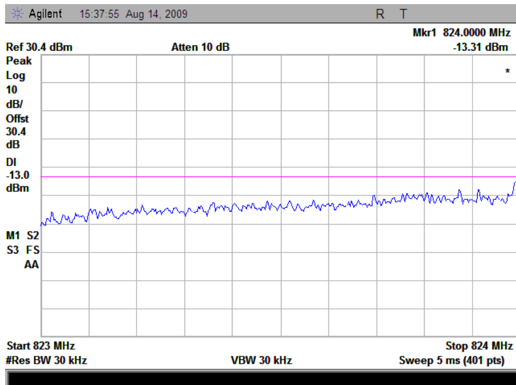
(Plot C: EVDO Channel = 1013)
