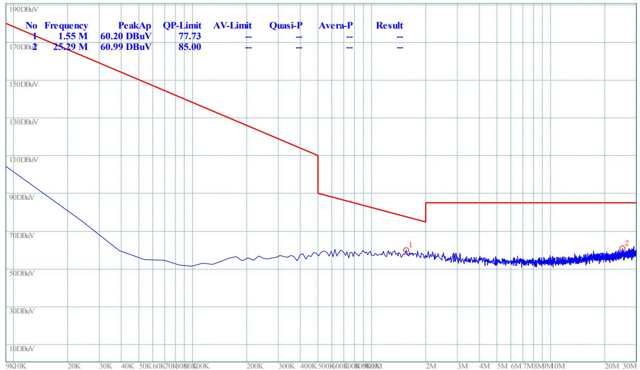
(Plot C.0: 9kHz to 30MHz @ GFSK, channel 78)
