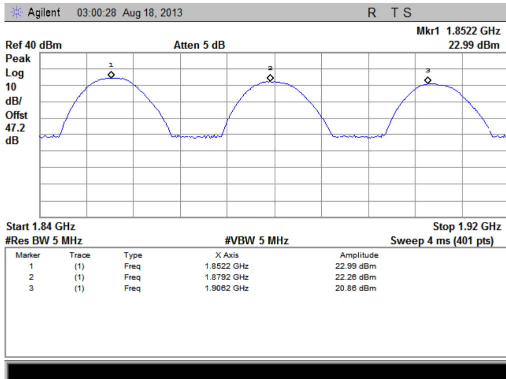
(Plot G: WCDMA 1900 MHz Channel = 9262, 9400, 9538)
