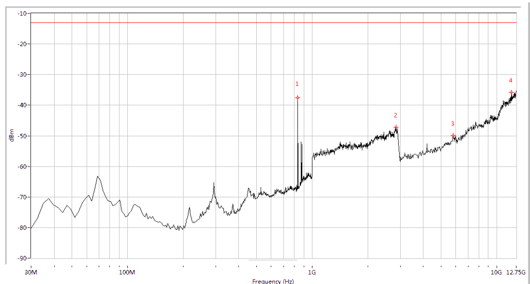
(Plot A.3: GSM850MHz Channel = 190, Test Antenna Horizontal)
