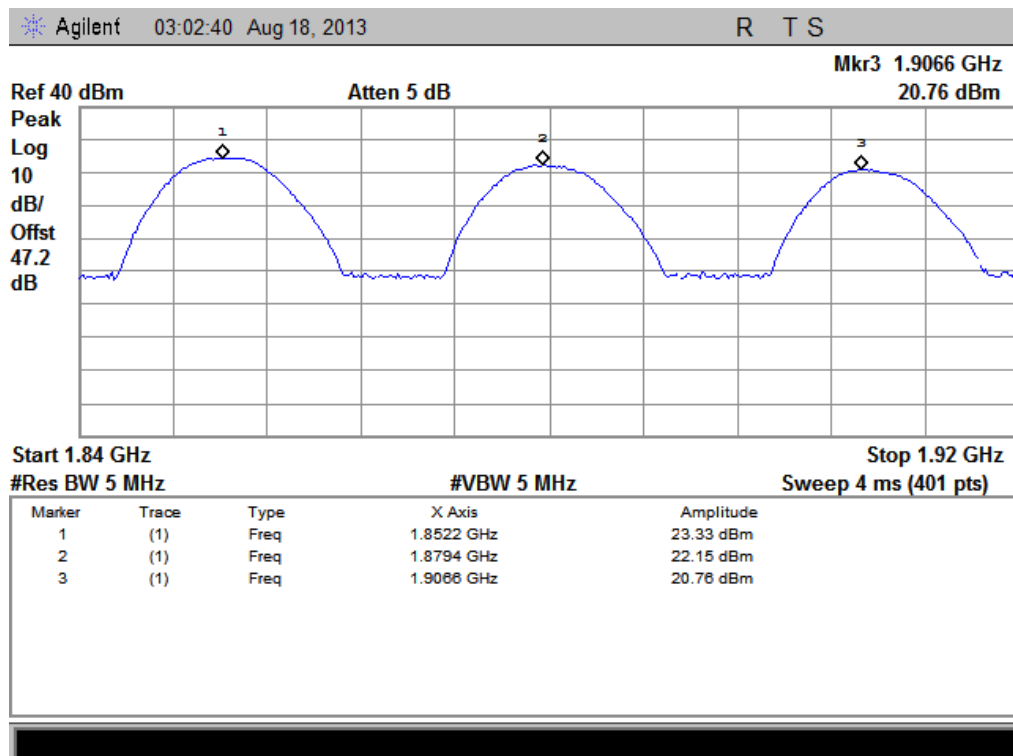
(Plot H: HSDPA1900 MHz Channel = 9262, 9400, 9538)
