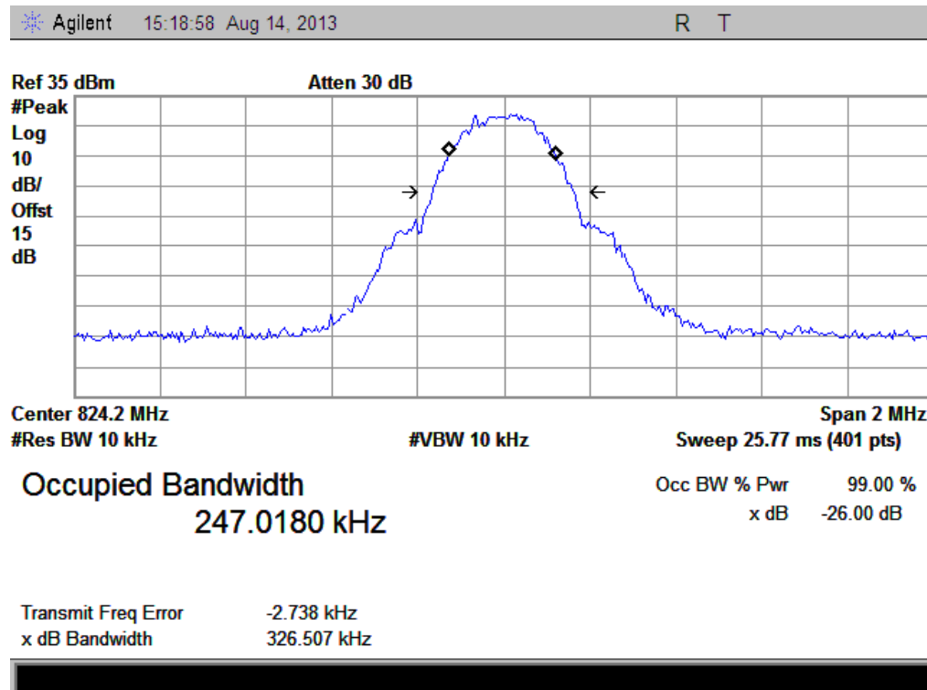
(Plot S: GPRS 850MHz Channel = 128)
