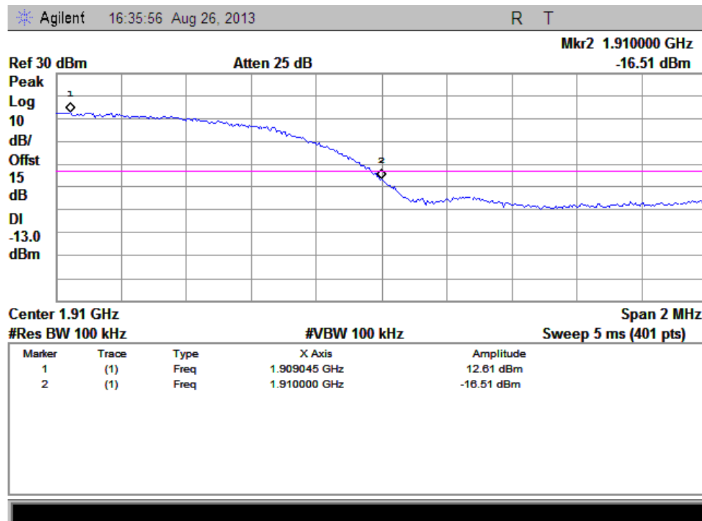
(Plot L: HSDPA 1900 Channel = 9538)
