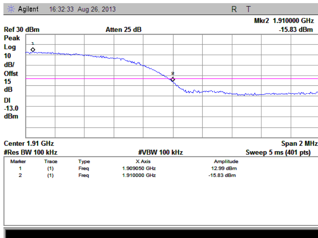
(Plot H: WCDMA 1900 Channel = 9538)
