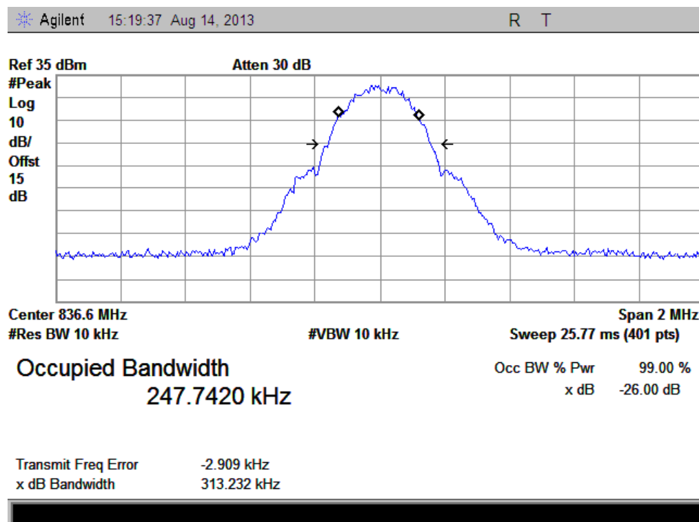
(Plot T: GPRS 850MHz Channel = 190)
