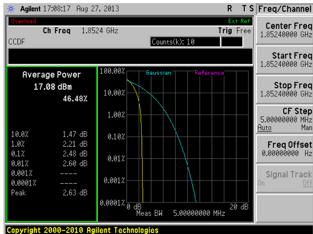
(Plot B1: WCDMA 1900MHz Channel = 9262)
