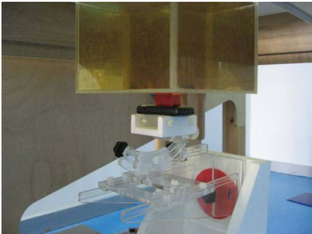
Fig.9 Side Position
