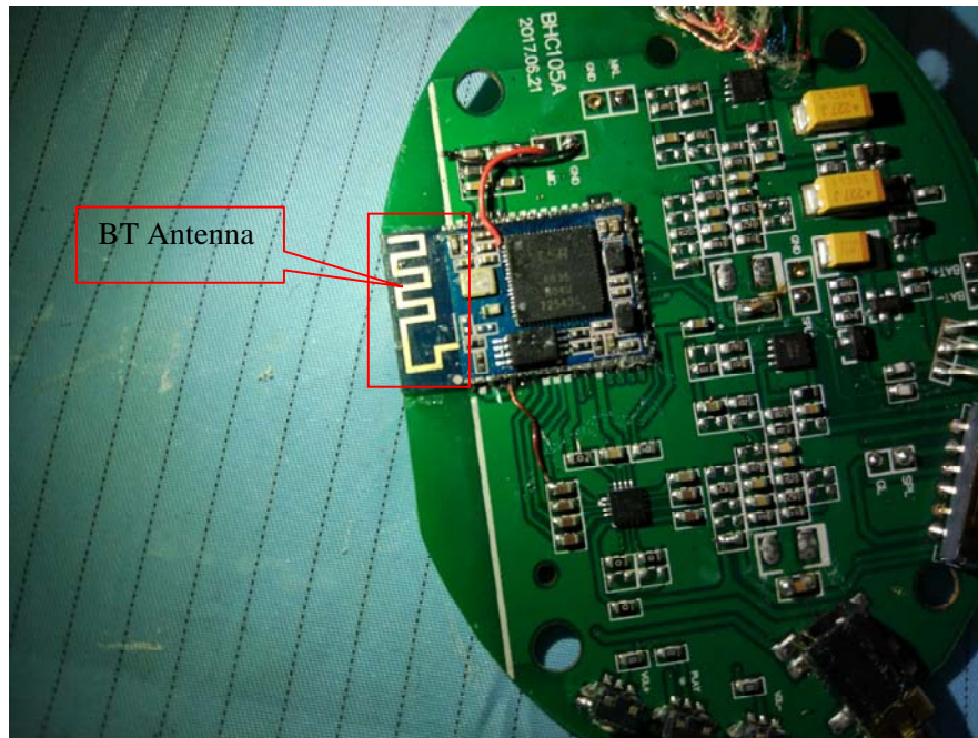
EUT – IC & Antenna View
