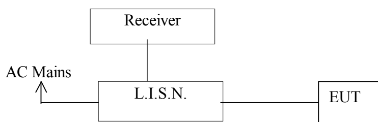
Figure 1 Conducted Disturbance Test Setup
