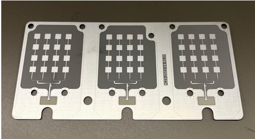
Figure 11 Antenna Board EU23-2022-04-R Front
