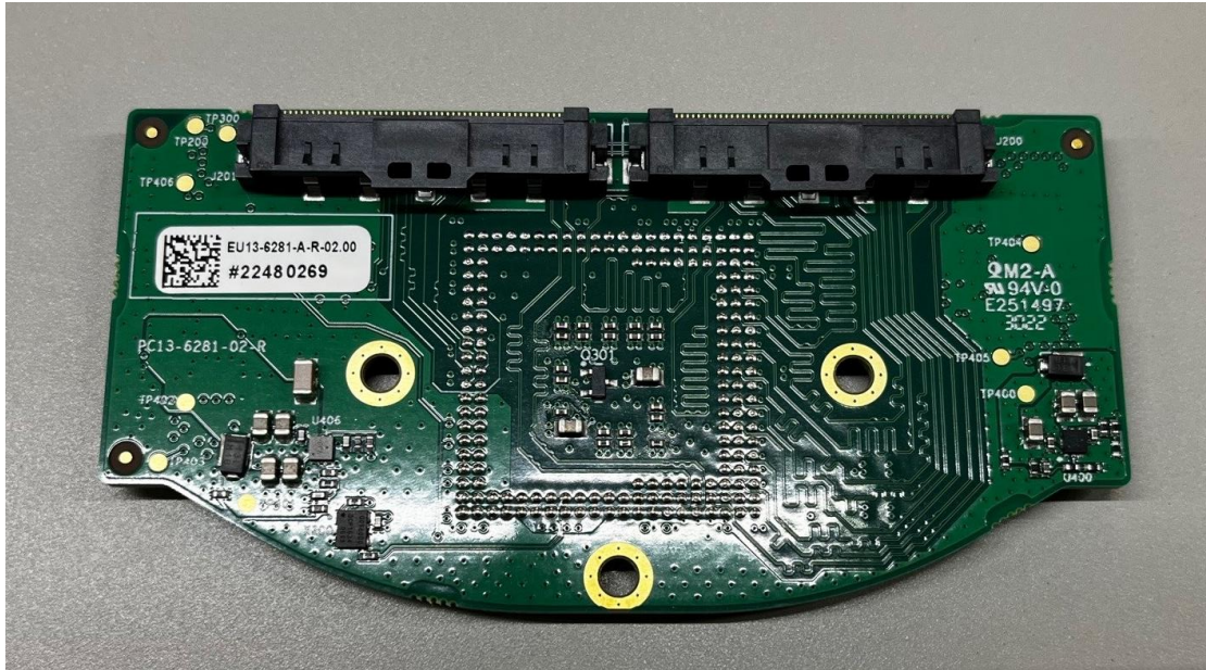
Figure 3 Sensor Board EU13-6281-A-R Front
