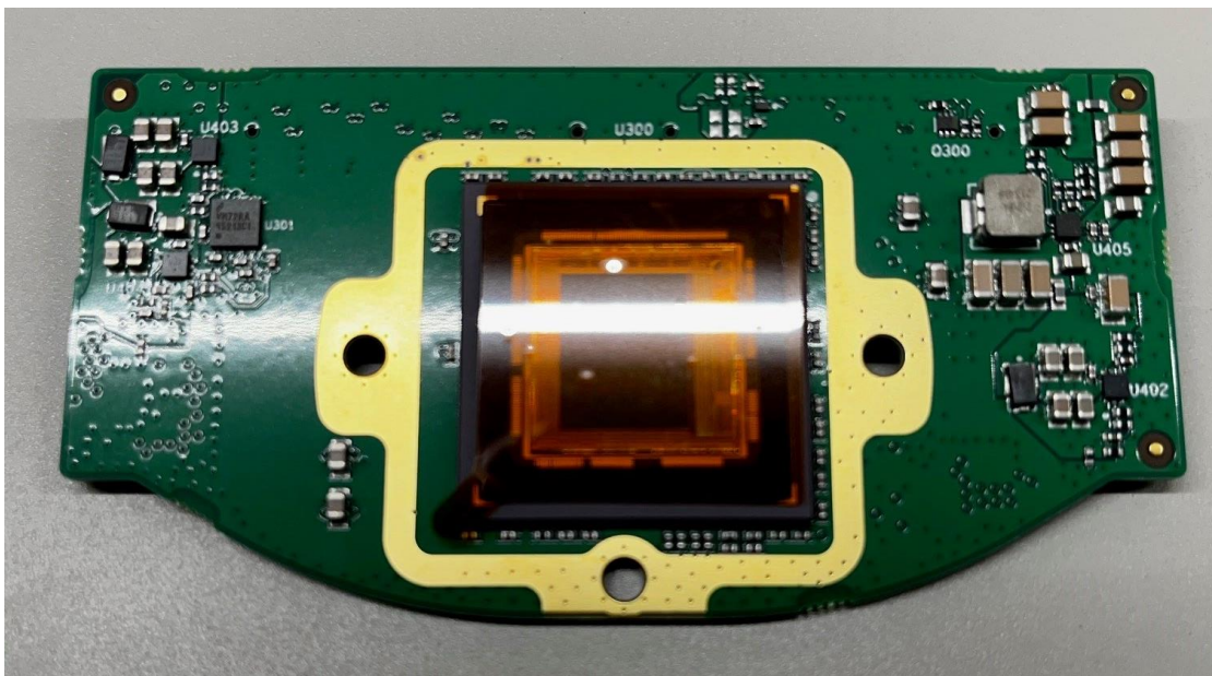
Figure 4 Sensor Board EU13-6281-A-R Back
