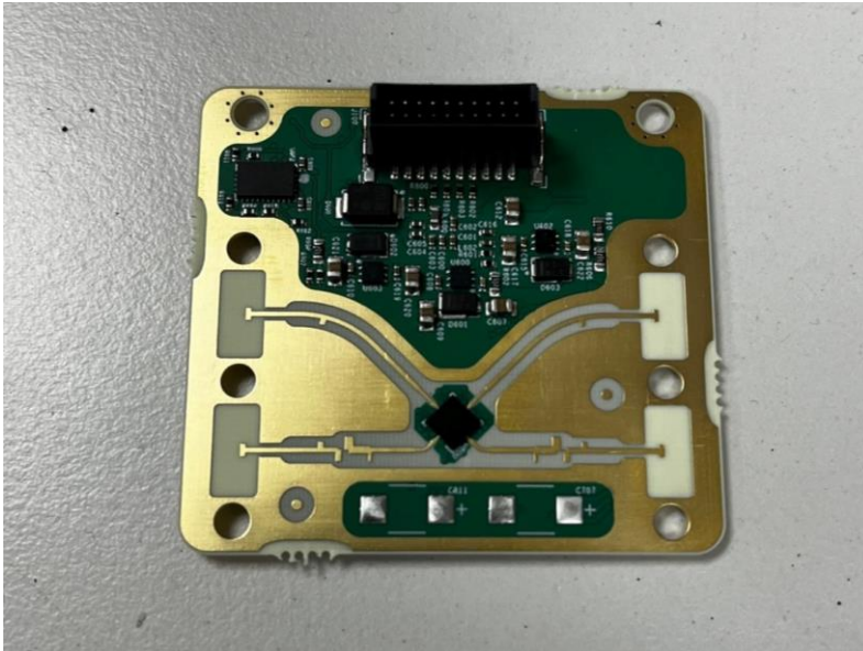
Figure 9 kRCM EU23-2020-A-R Front
