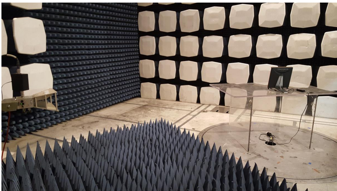
Photograph 3. Radiated Spurious Emissions, Test Setup, Above 1GHz
