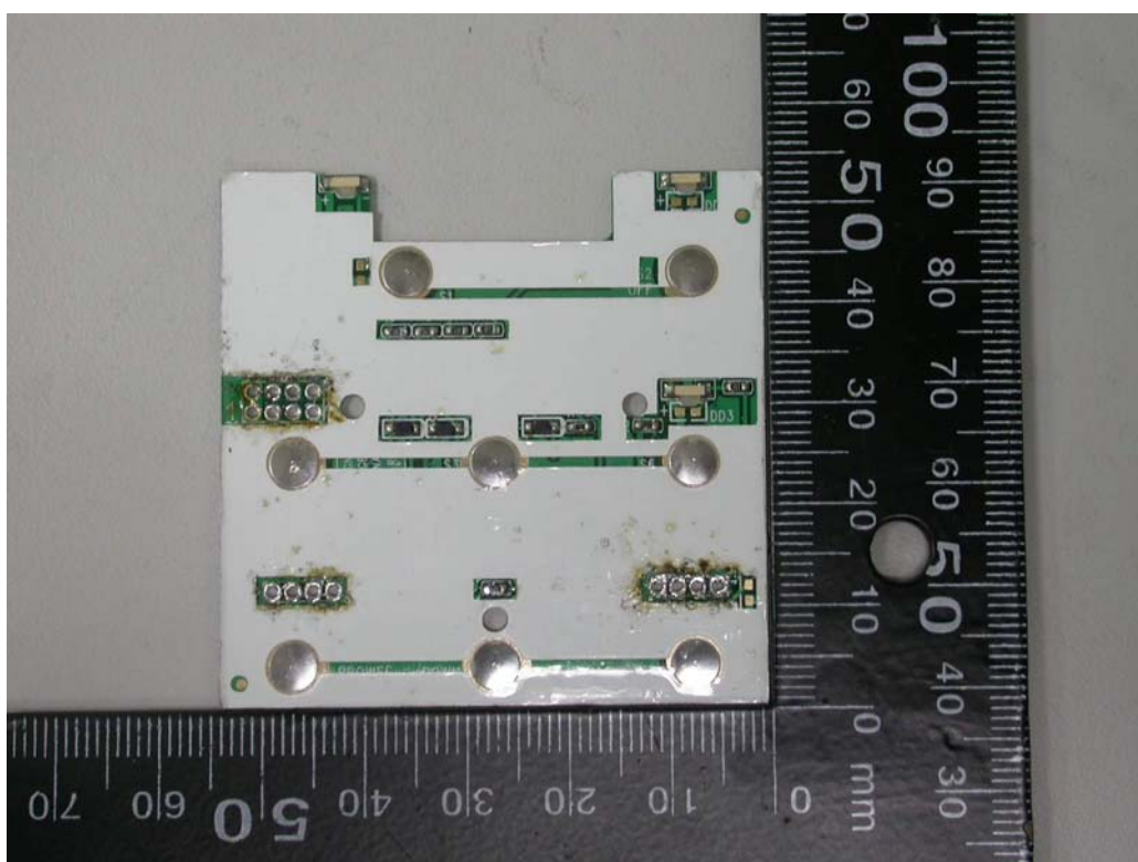
14. Front view of PCB3
