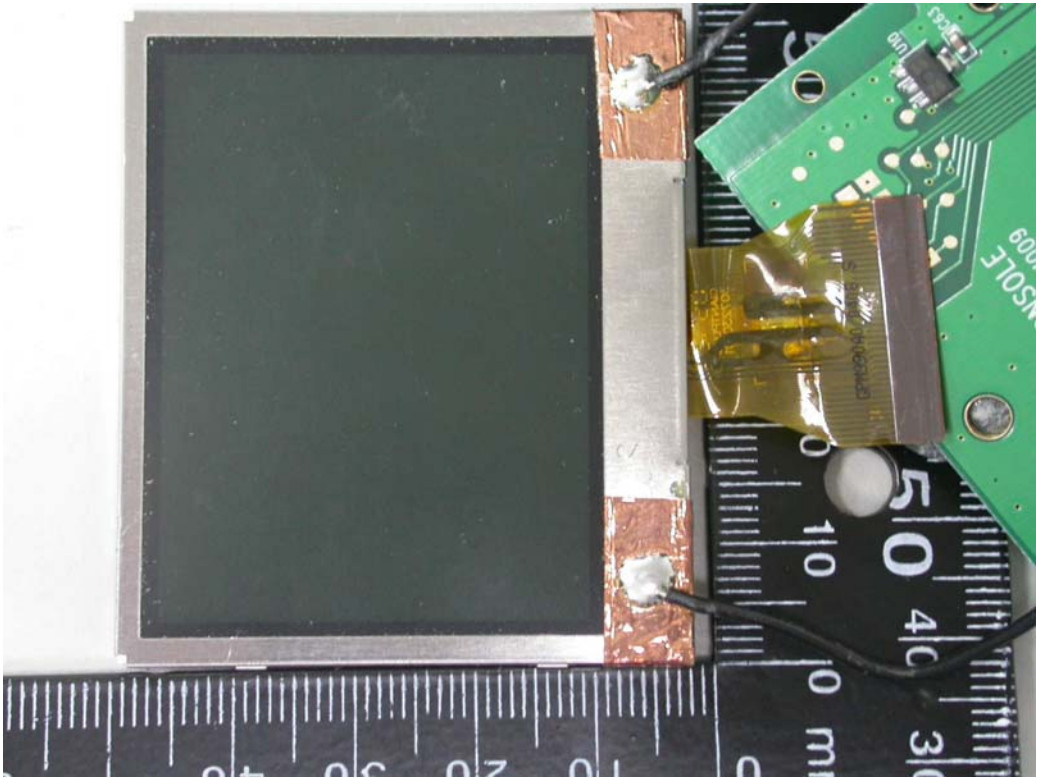
17. Front view of PCB4
