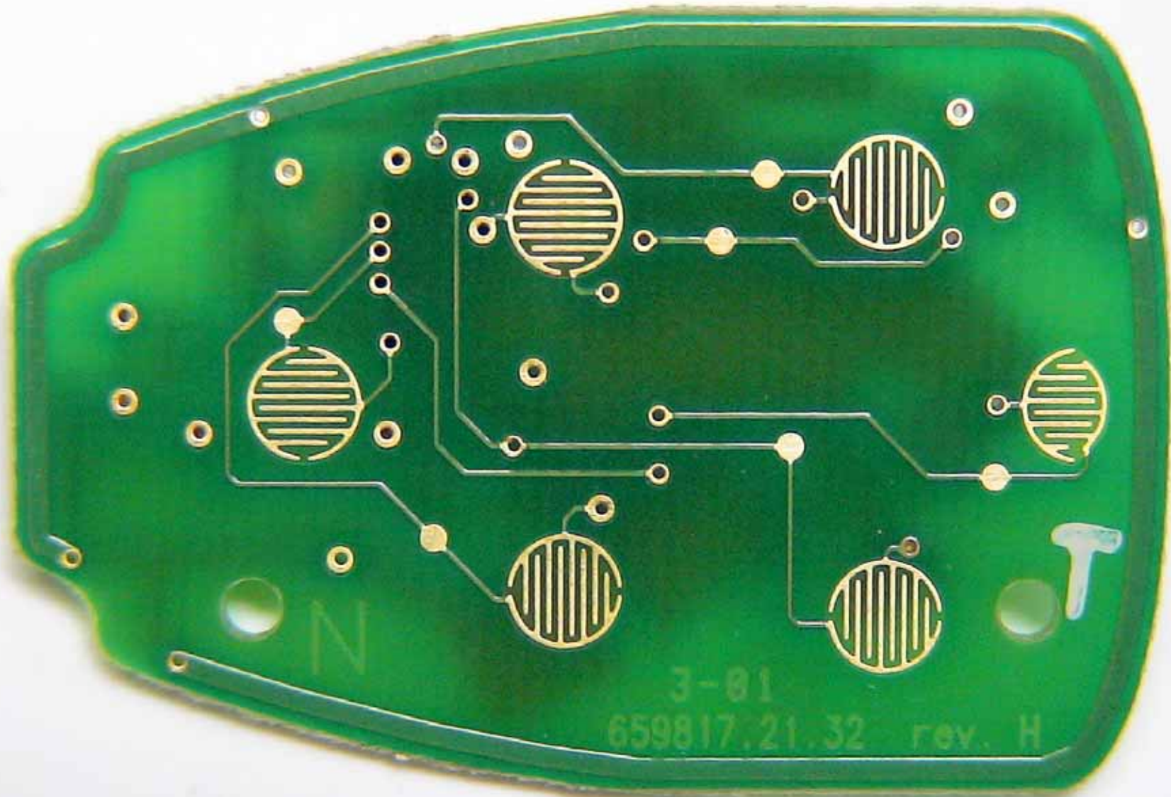
PCB (bottom)
