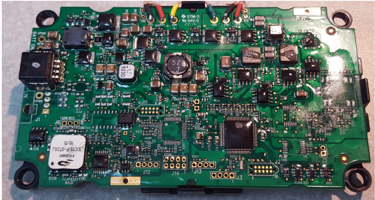
PC Board - Bottom
