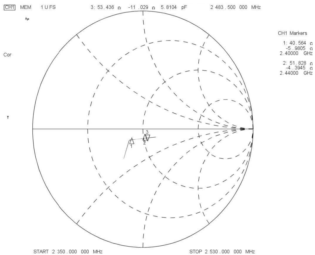
Fig. 3. Smith Chart
