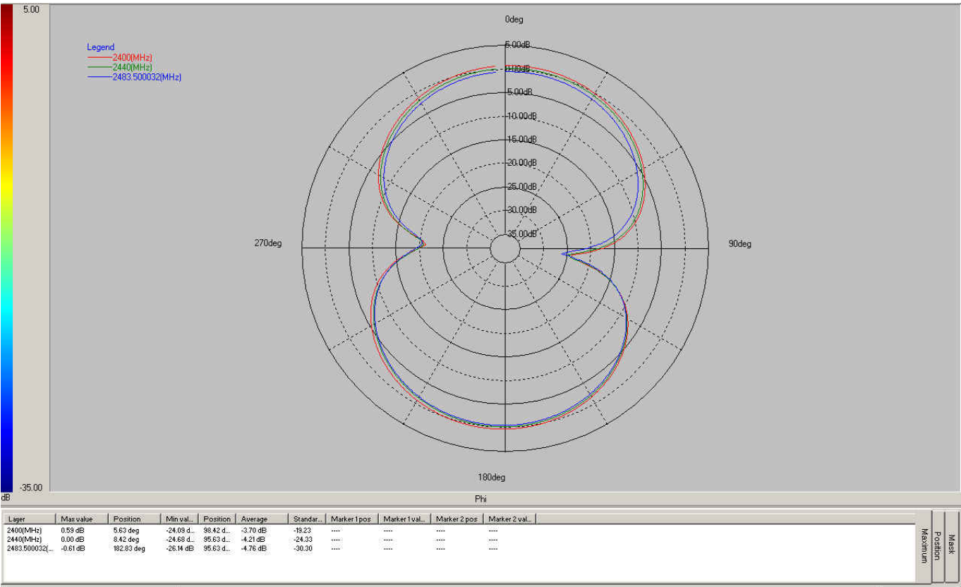
Elevation Pattern
