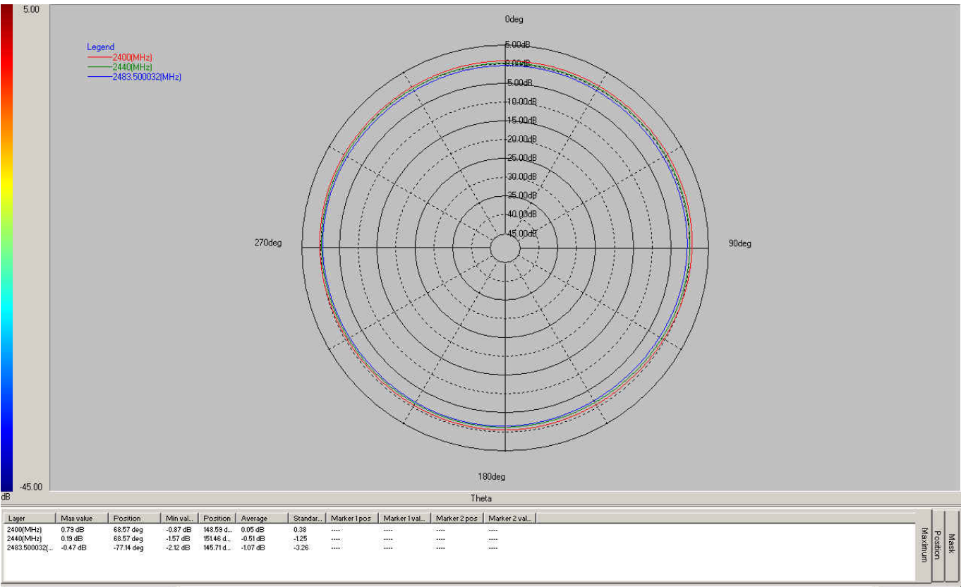
Azimuth Pattern
