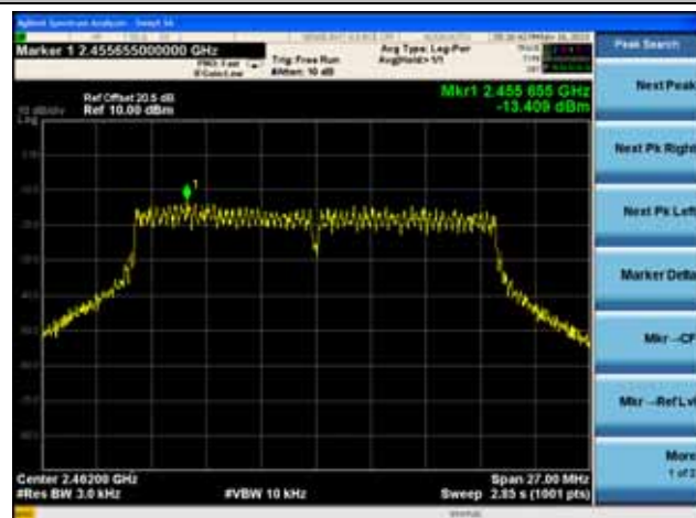
802.11n-HT20 PSD – Chain C
