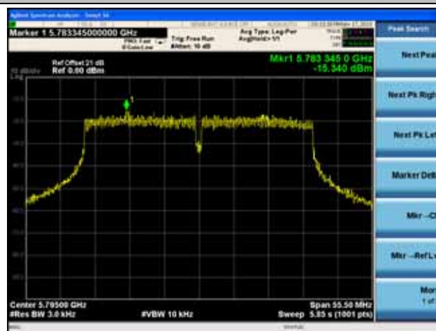
Channel 159 (5795MHz)
