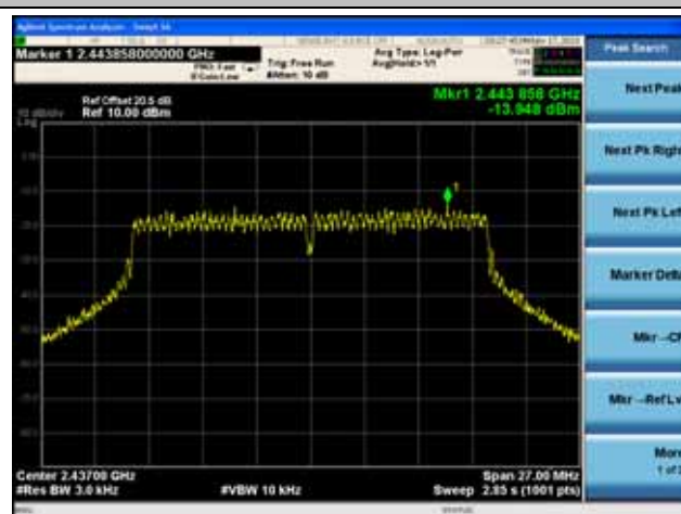
Channel 06 (2437MHz)
