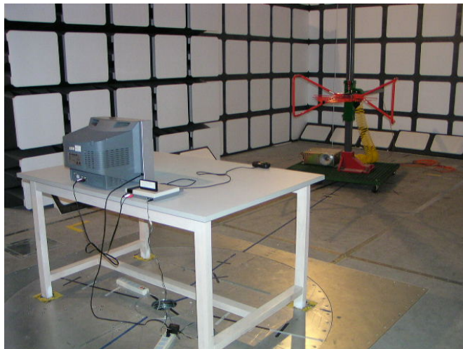
30 MHz-1GHz: Radiated Emissions-Rear View
