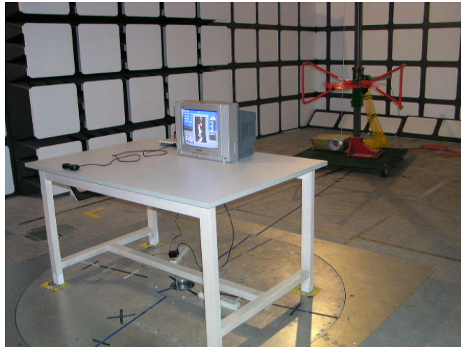
30 MHz-1GHz: Radiated Emissions-Front View
