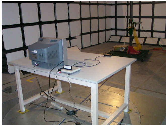
1 GHz-25GHz: Radiated Emissions-Rear View
