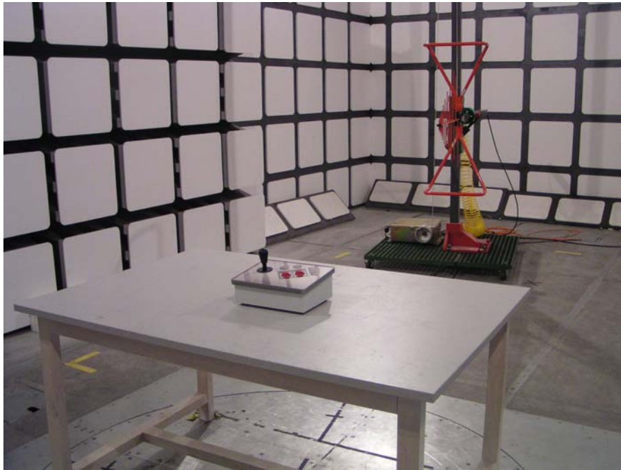
30 MHz – 1000 MHz: Radiated Emissions - Front View
