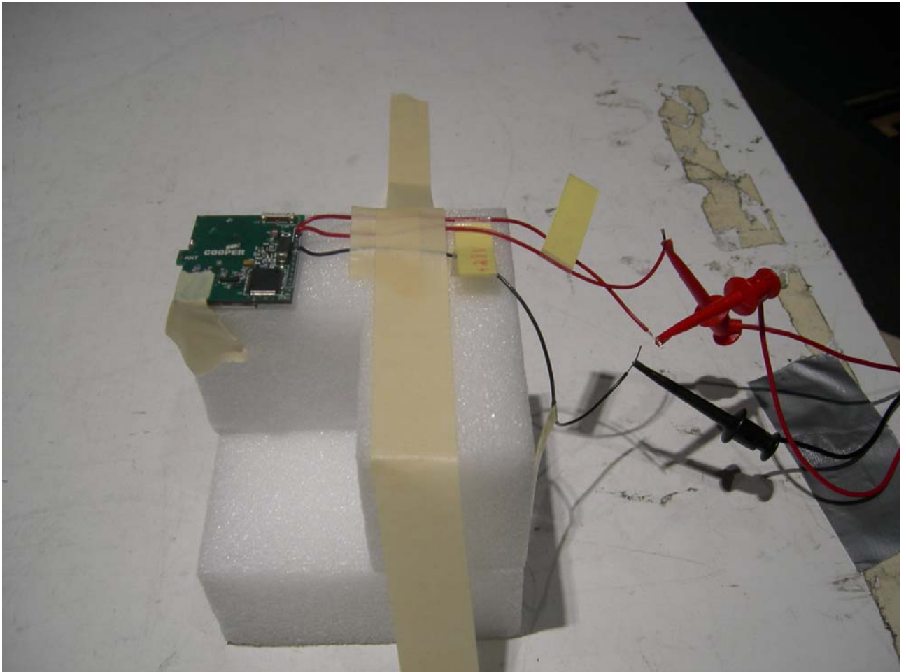
Figure 2: Radiated Emissions – Intentional – Close Up View
