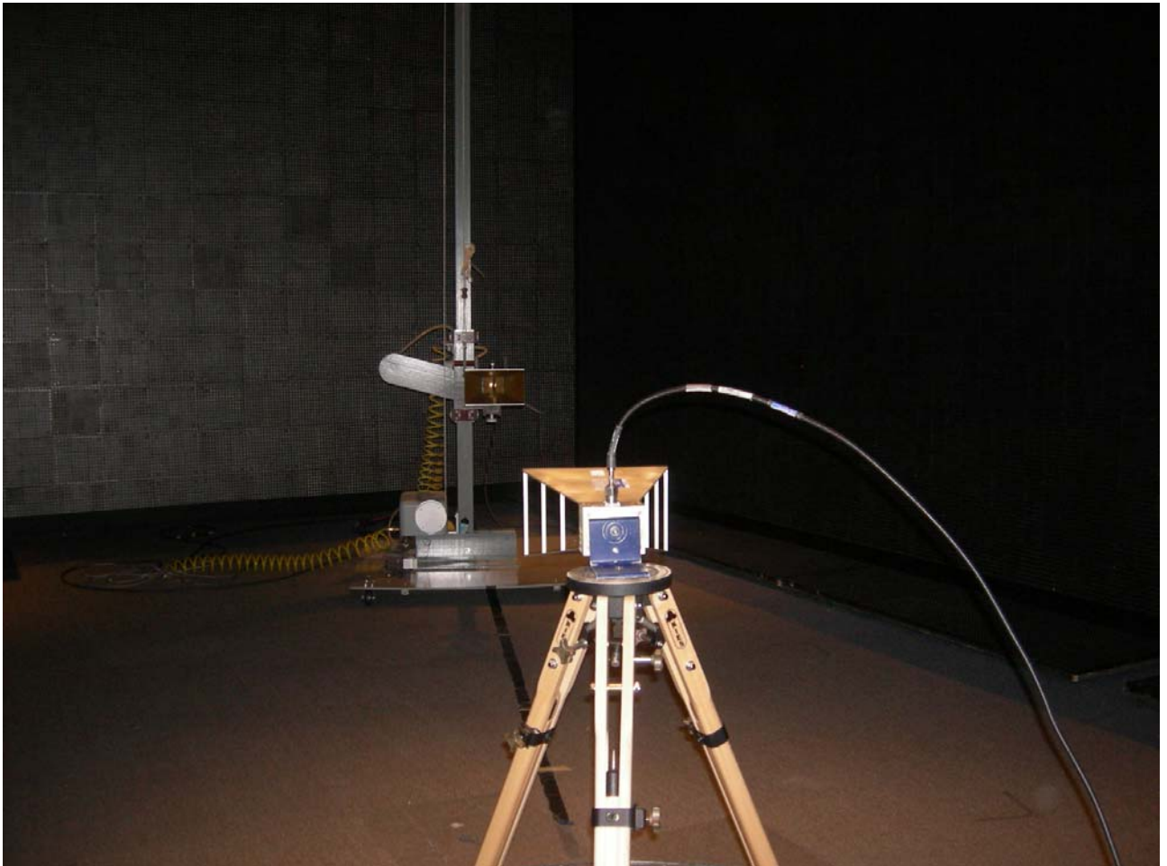
Figure 3: Radiated Emissions – Substitution
