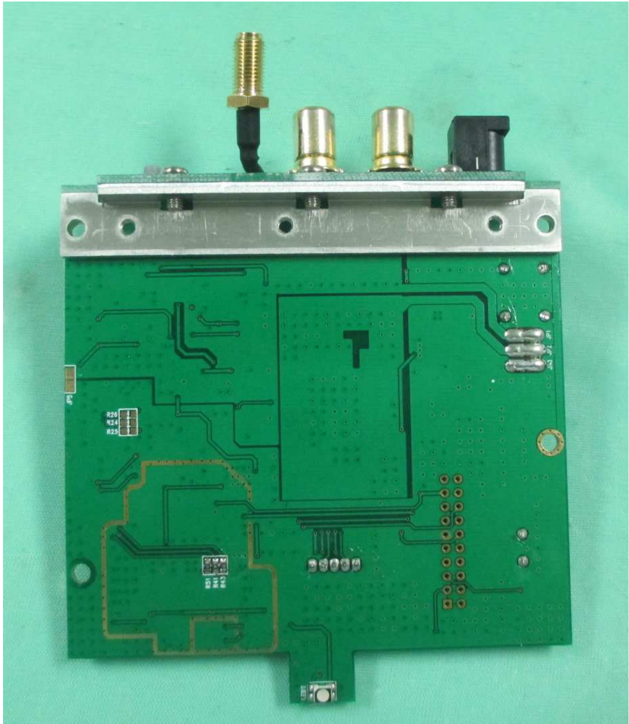
PHOTOGRAPH OF THE PRODUCT INNER CIRCUIT BOTTOM VIEW
