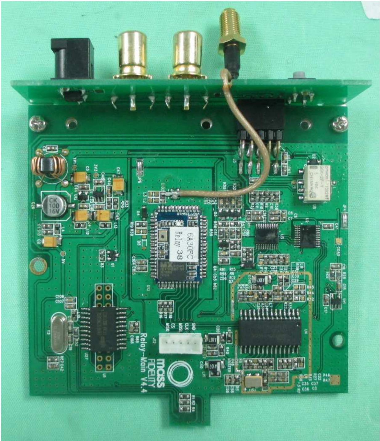
INNER CIRCUIT TOP VIEW
