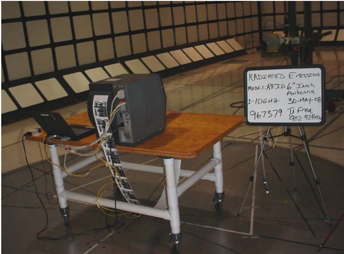
Test Set Up Radiated Emissions 1-10GHz Rear View
