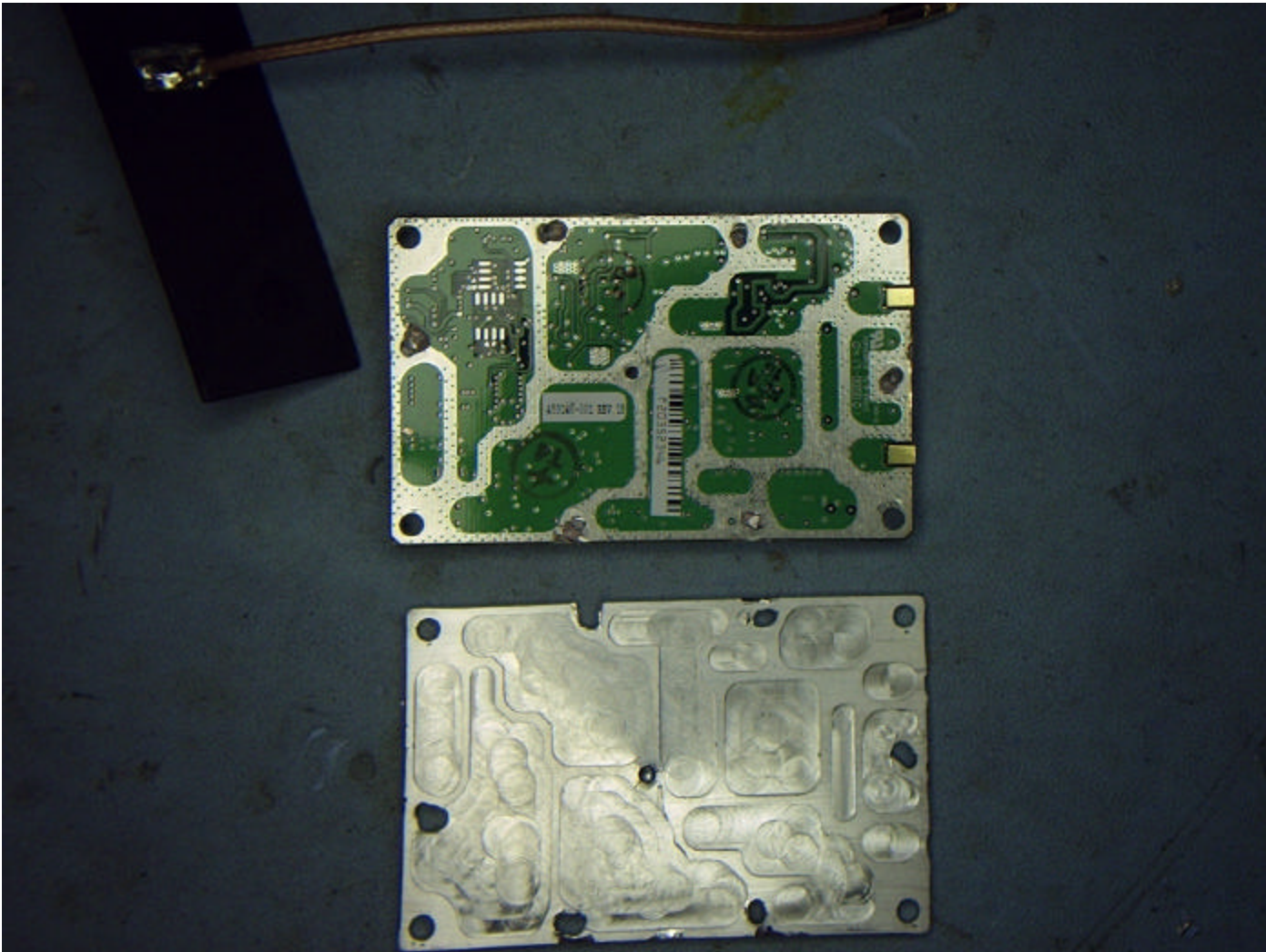
Internal Photos - Solder Side (with Cover)
