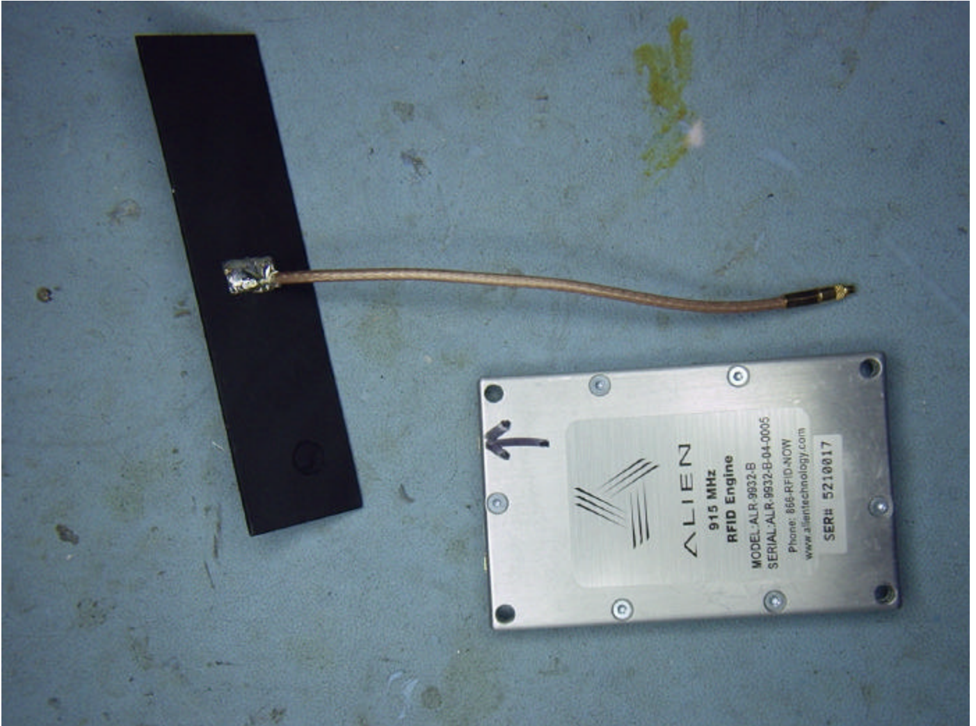
External Photo - Top Side with Antenna
