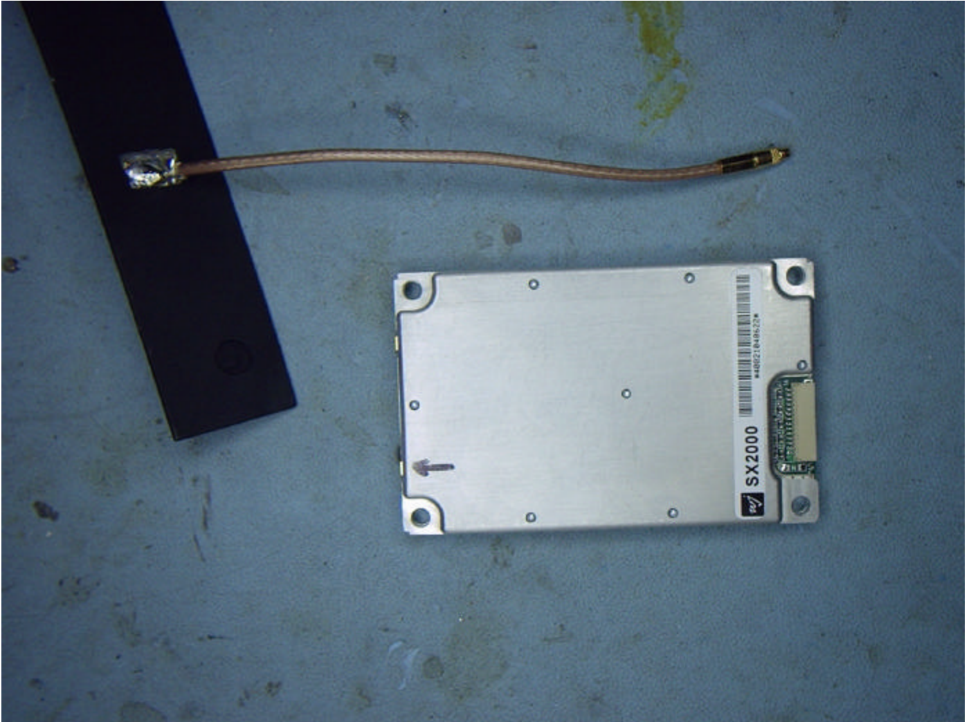
External Photos - Bottom Side with Antenna
