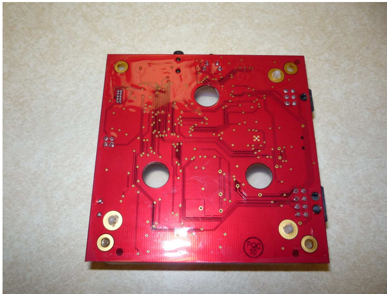
Figure 4 ZpassV2 Bottom
