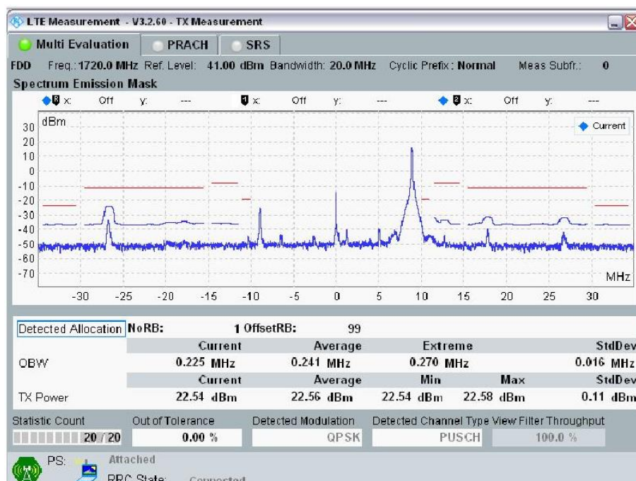
20MHz Band Width: Ch 20050, RB Size=1; RB Offset = 99
