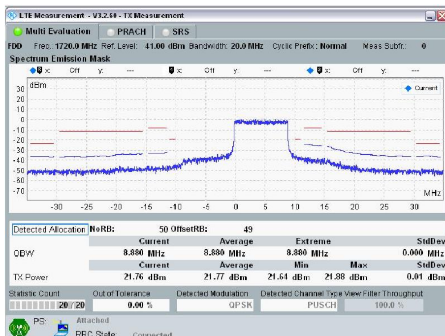
20MHz Band Width: Ch 20050, RB Size=50; RB Offset = 49
