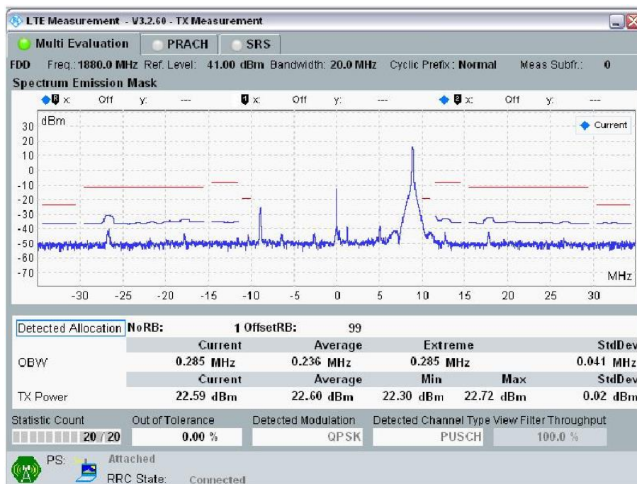
20MHz Band Width: Ch 18900, RB Size=1; RB Offset = 99
