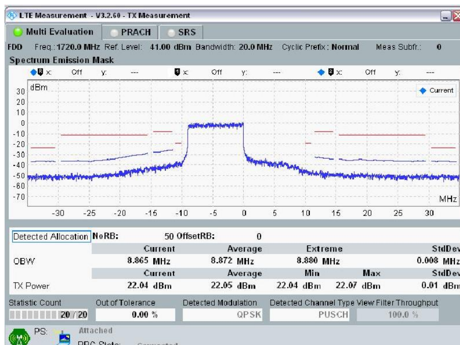
20MHz Band Width: Ch 20050, RB Size=50; RB Offset = 0
