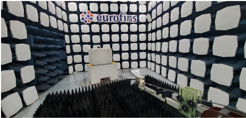
Picture 1 Radiated Spurious Emissions Test setup
