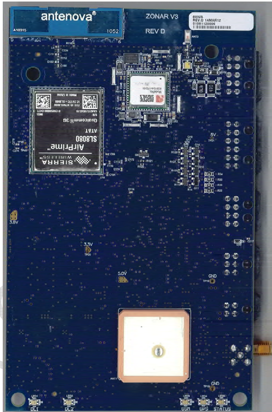
Figure 1 Antenna/Top side of V3 Device GSM antenna in the upper left
