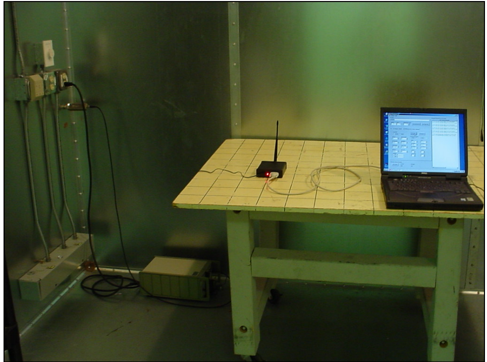
Setup for the Conducted Emissions Test
