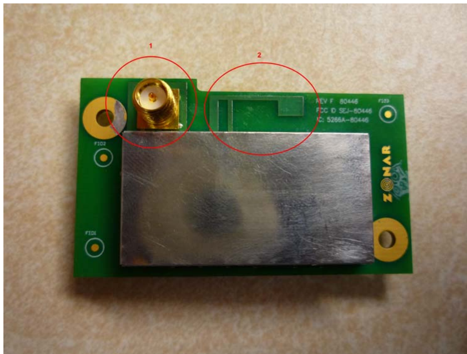
Figure 1 80446 uses either unique antenna connector or integrated trace antenna
