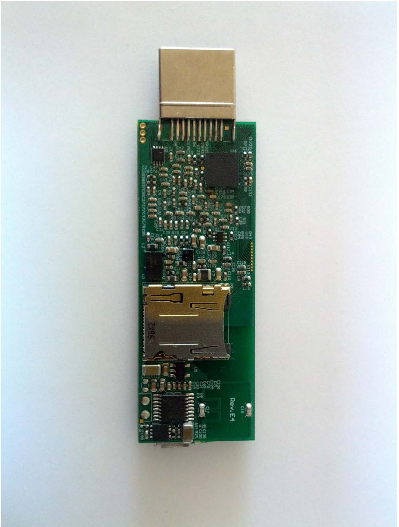
BOTTOM VIEW OF PCB
