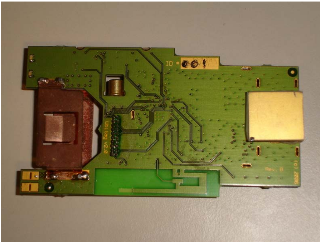
Solder Side
