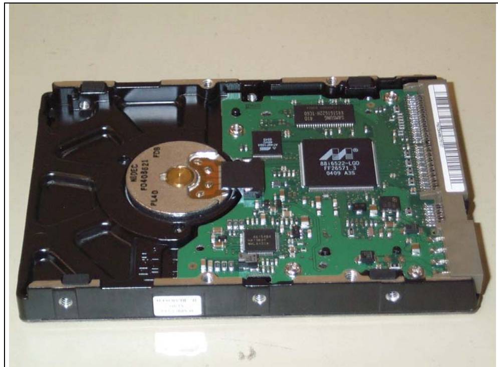
Picture 13. Harddrive
