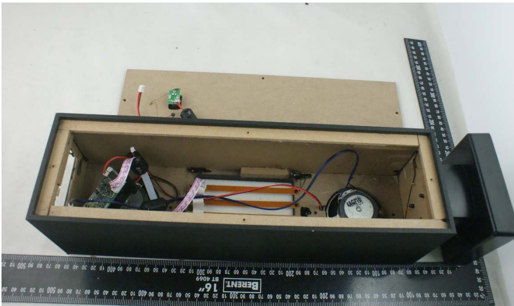
EUT UNCOVER VIEW 2
