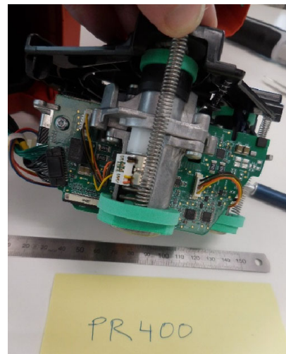
Main Board
