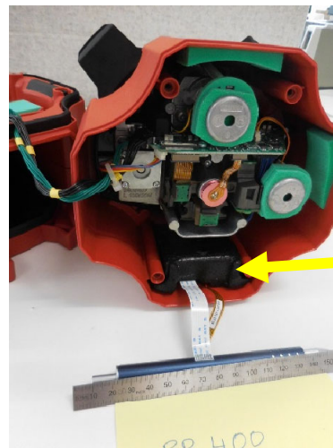
Sensor Board
