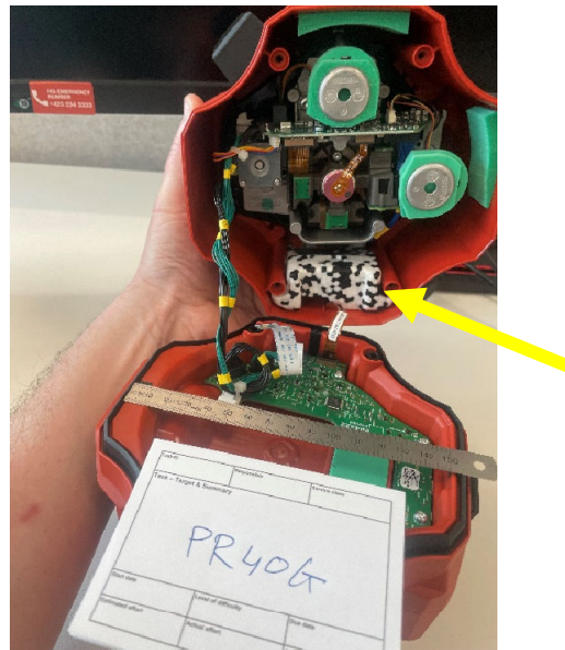
Location of BLE Board inside the tool
