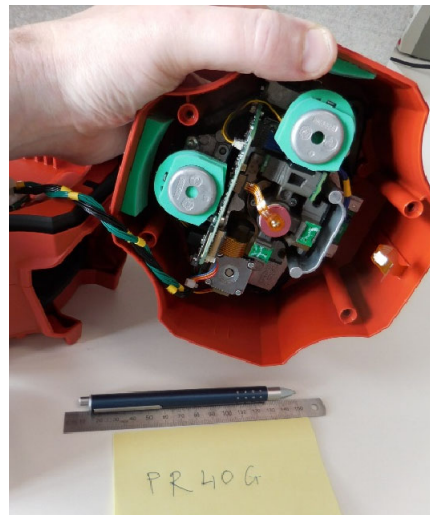
Sensor Board
