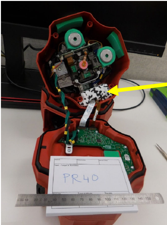
Opened tool / Sensor Board
