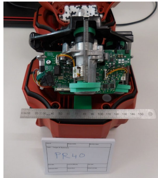
Main Board
