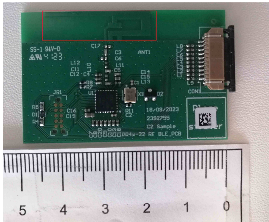
(top view – PCB Antenna)
