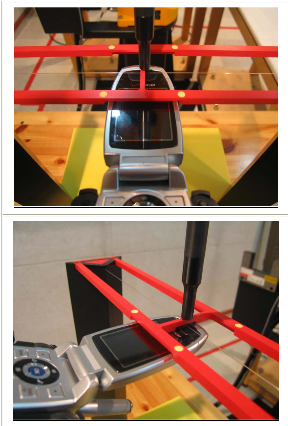
Figure 4. Test Set-up Photo
