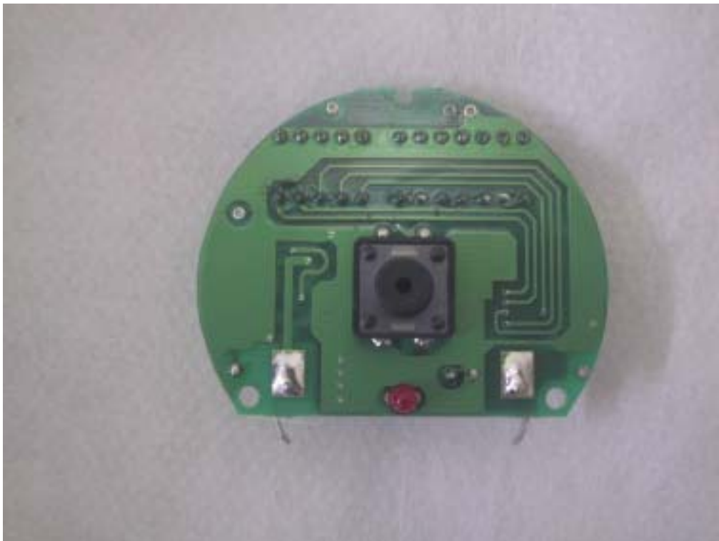
Rear of EUT (Internal)
