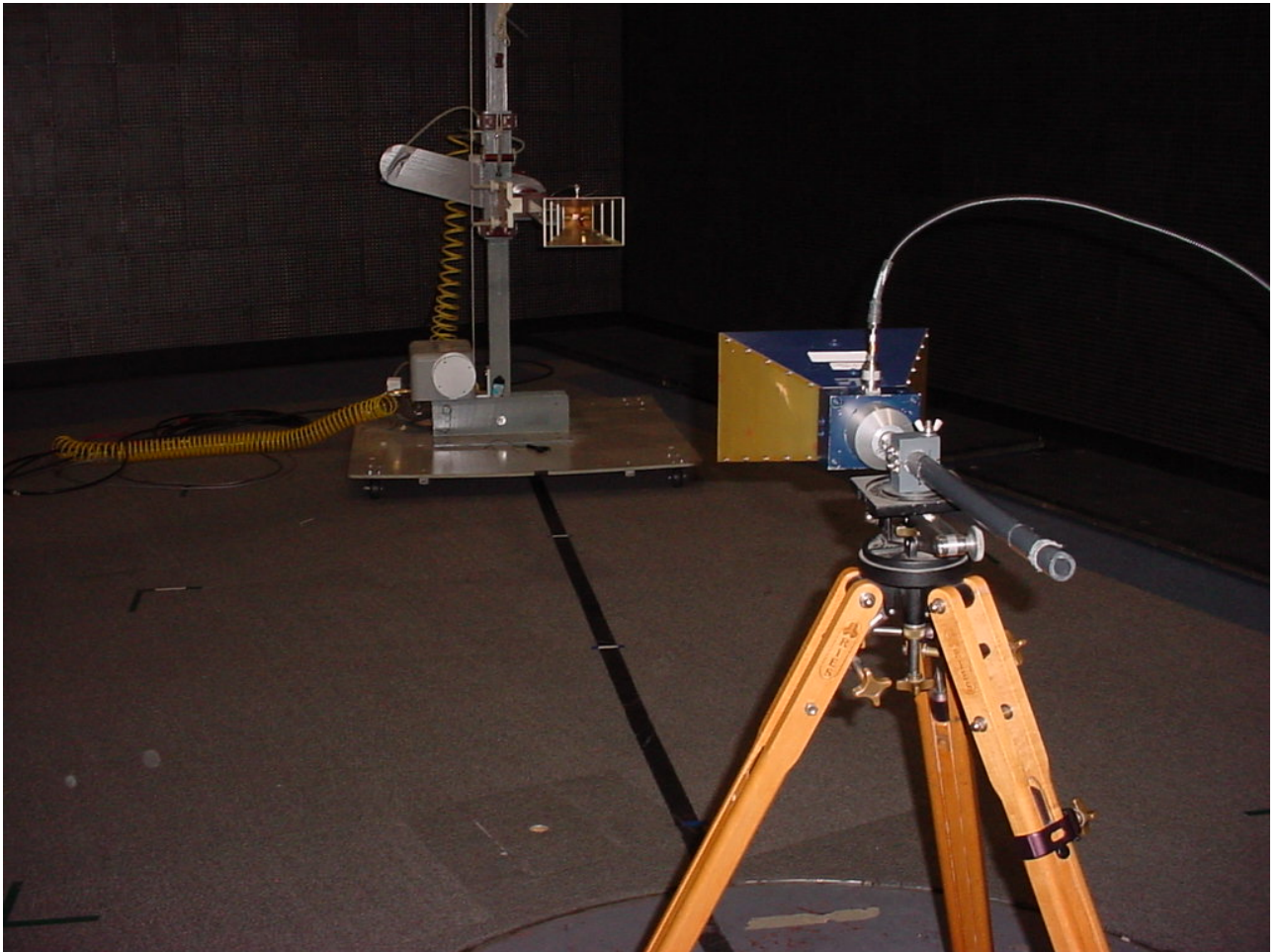
Figure 3: Intentional Radiated Emissions – Substitution
