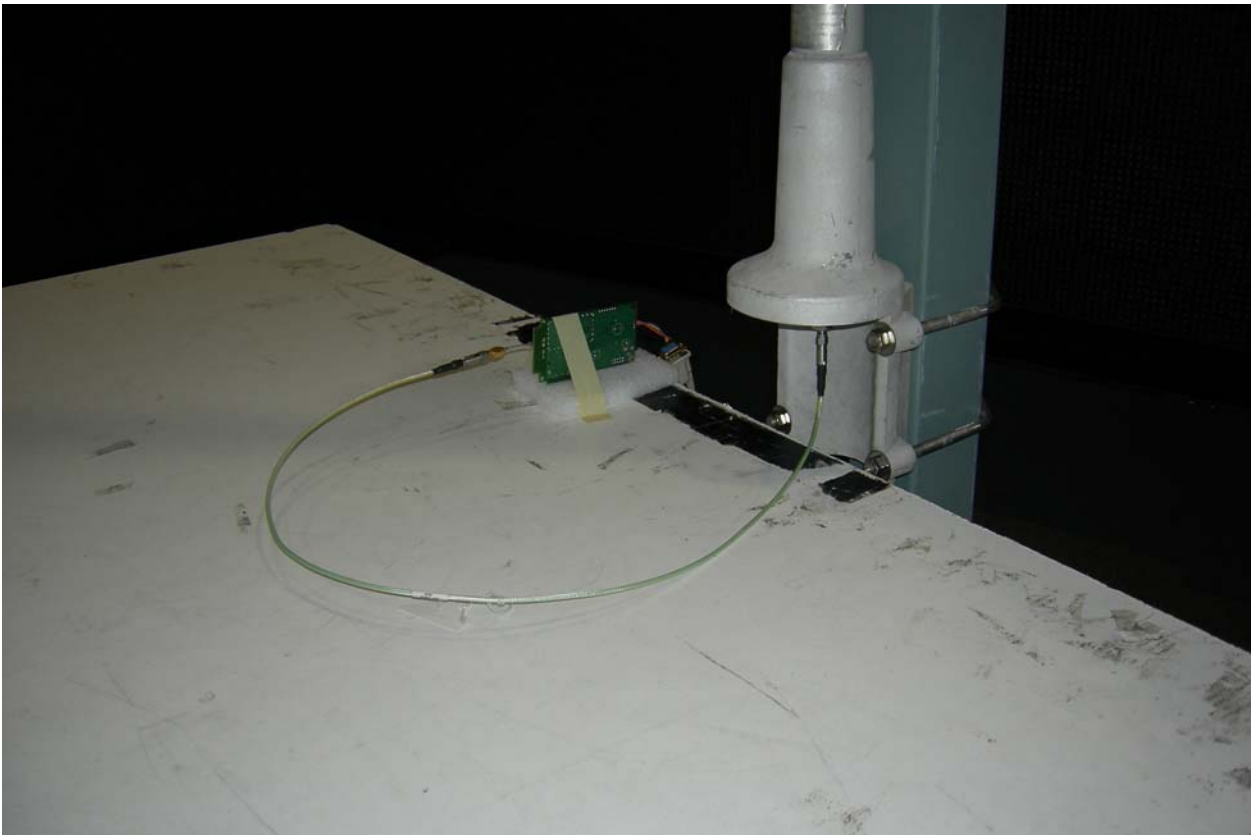
Figure 4: Unintentional Radiated Emissions – External Antenna.
