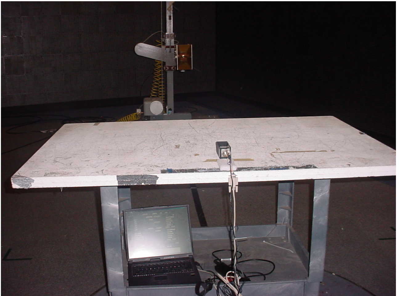
Figure 1: Intentional Radiated Emissions
