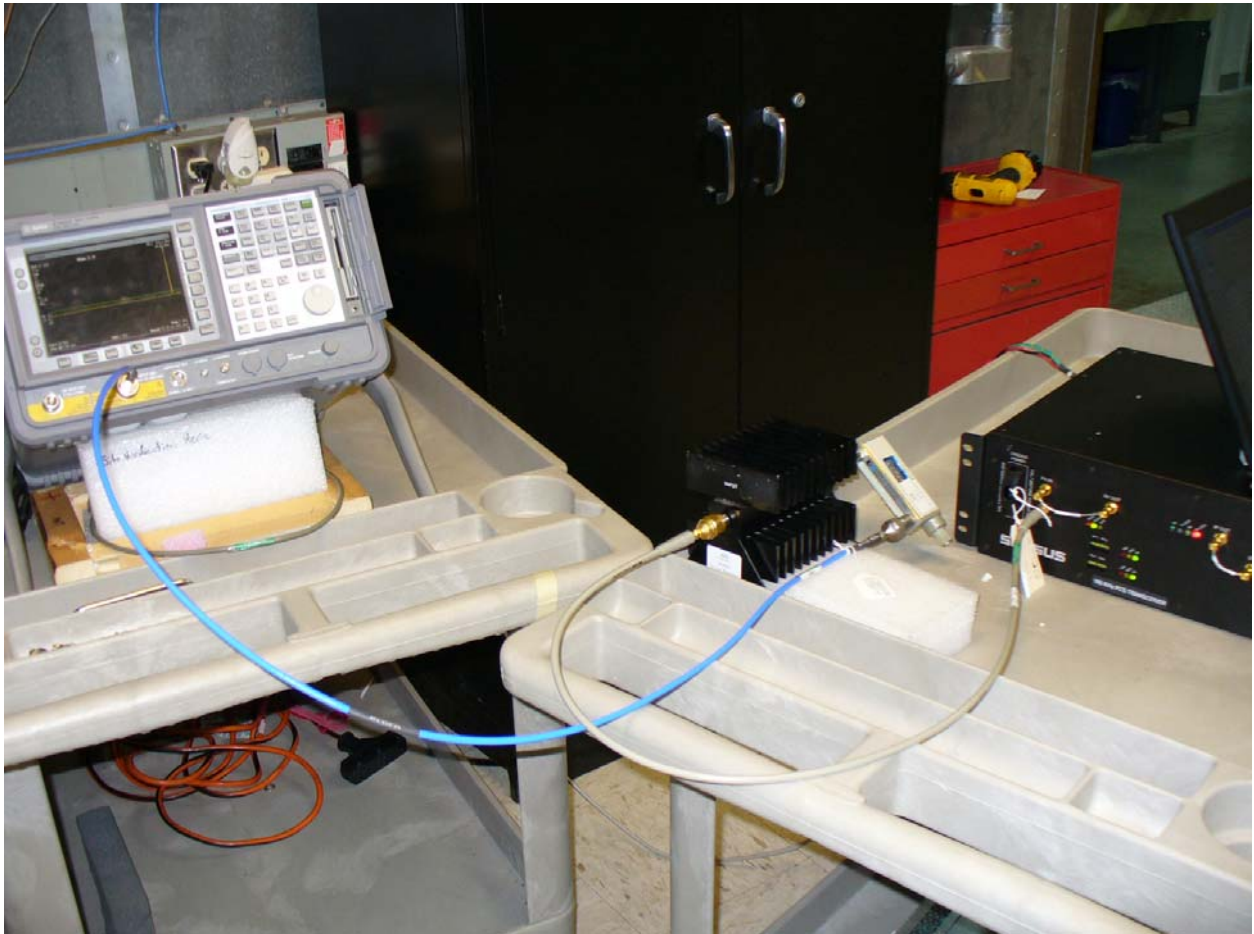
Figure 3: RF Conducted Emissions (Set Up 1)
