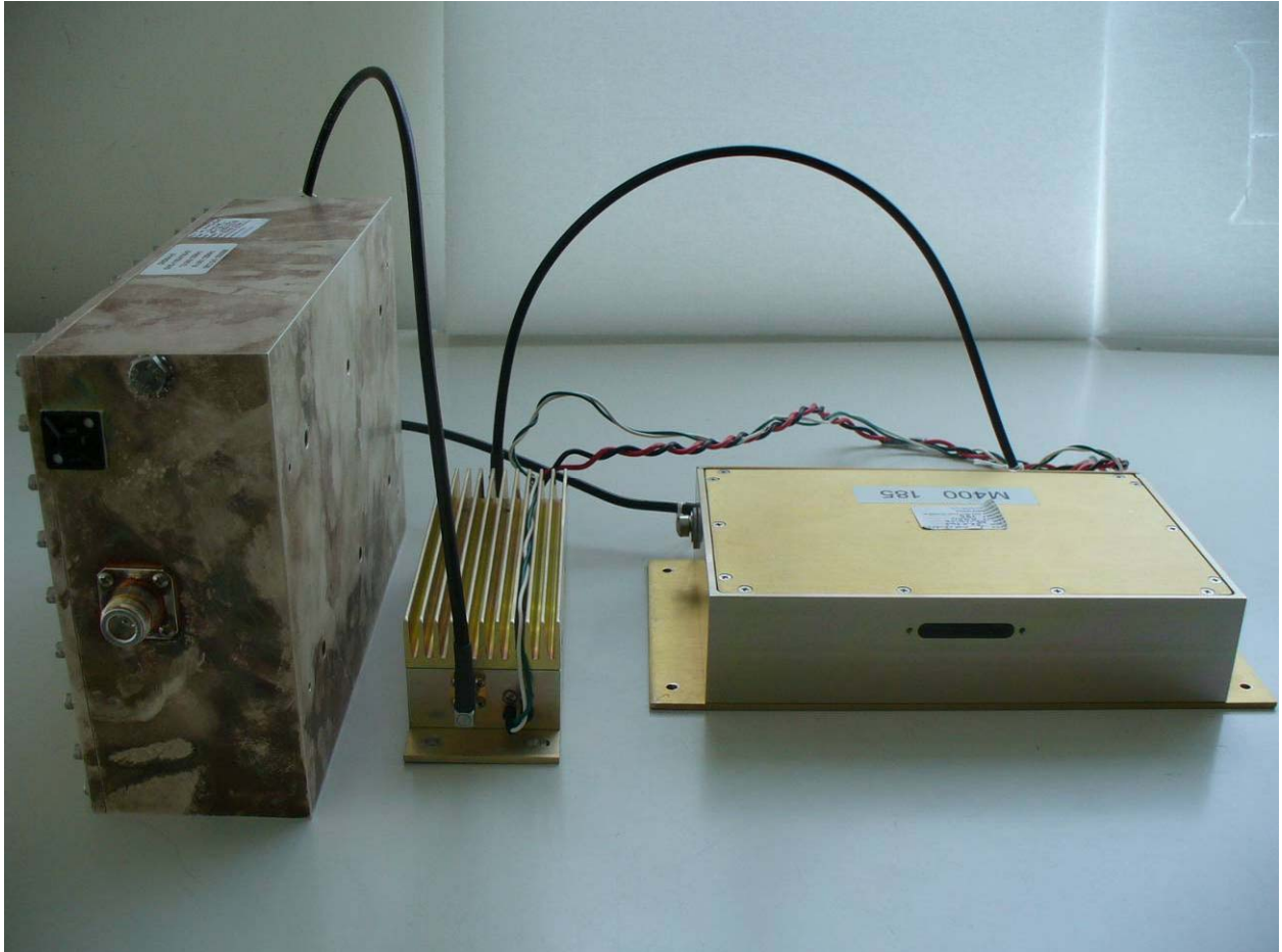
Figure 21: M400XCVR-01, Power Amplifier and Duplexer (Assembled – Rear View)
