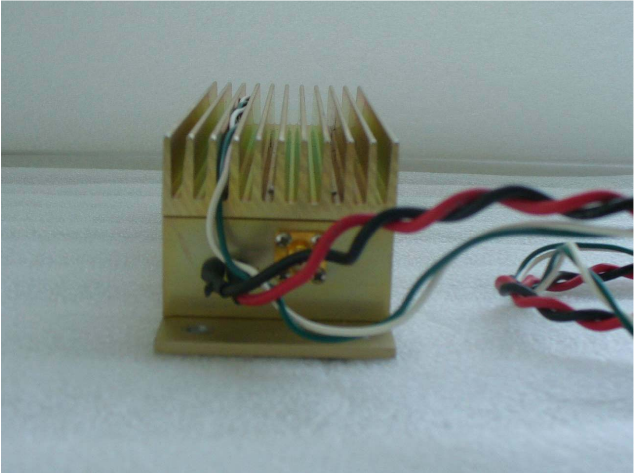
Figure 16: Power Amplifier (Rear View)
