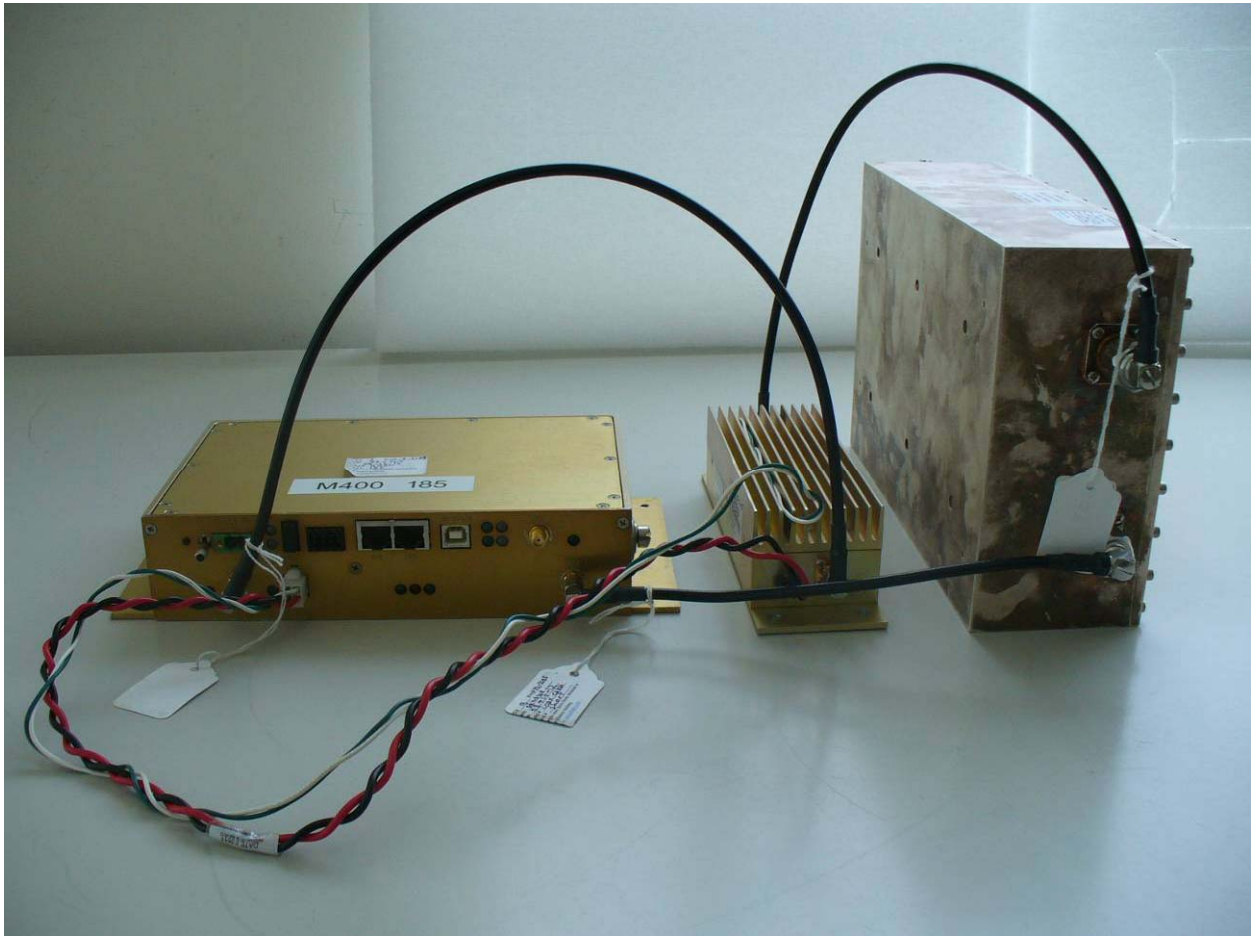
Figure 20: M400XCVR-01, Power Amplifier and Duplexer (Assembled – Front View)
