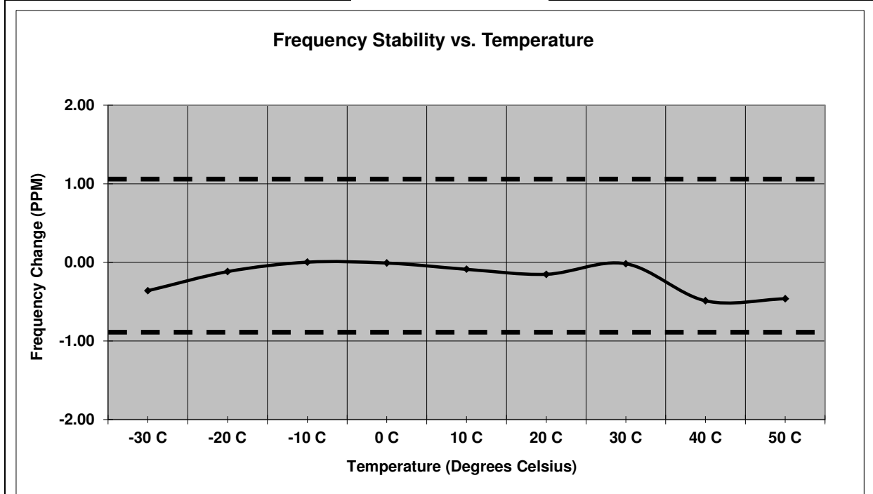
Figure 7.6.2-7: Frequency Stability – 959.925 MHz – KDS
