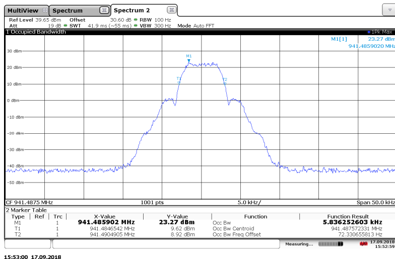
Figure 7.3.2-39: 941.4875 MHz – MPass 5k Mode
