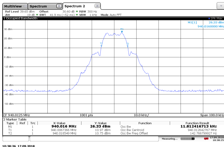
Figure 7.3.2-16: 940.0125 MHz – MPass 10k Mode
