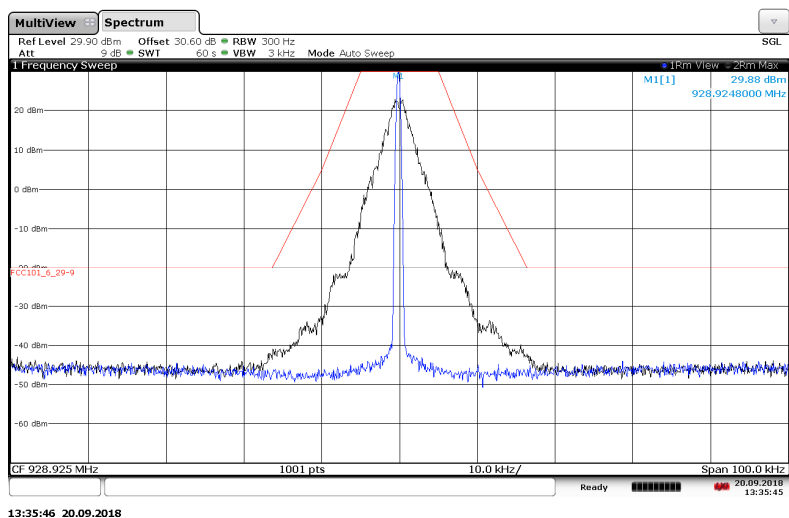
Figure 7.2.2-22: 928.925 MHz – 25 kHz Channel Spacing – Priority Mode
