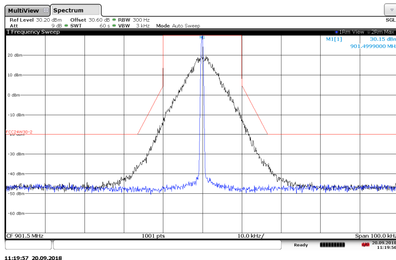
Figure 7.2.2-2: 901.5 MHz – 25 kHz Channel Spacing – Double Density Mode
