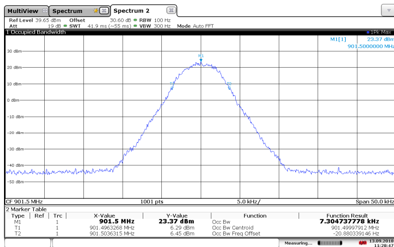
Figure 7.3.2-7: 901.5 MHz – 8SFSK (Half Baud) Mode
