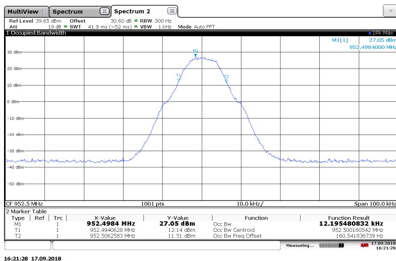
Figure 7.3.2-46: 952.5 MHz – M4Pass 20k Mode
