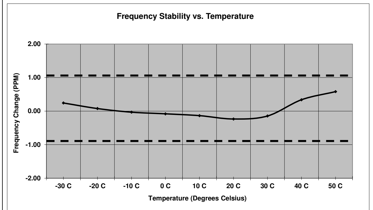
Figure 7.6.2-9: Frequency Stability – 959.925 MHz – EPSON
