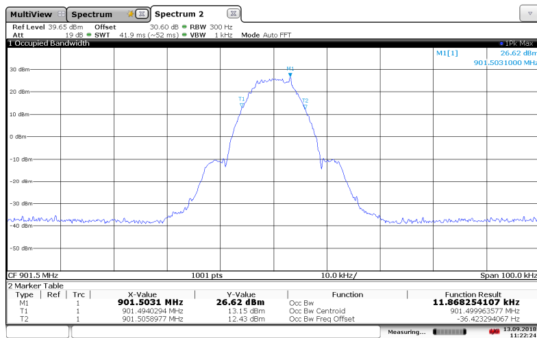
Figure 7.3.2-8: 901.5 MHz – 2SFSK Mode
