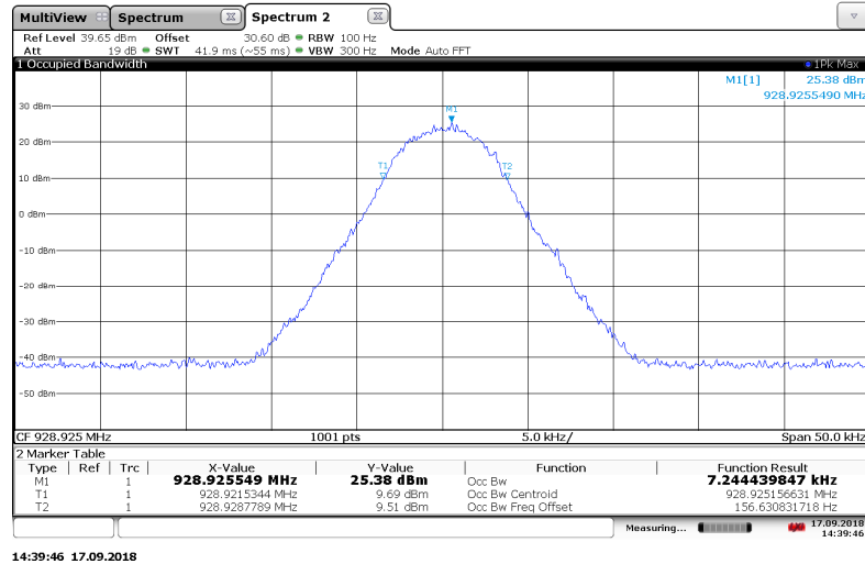
Figure 7.3.2-25: 928.925 MHz – 8SFSK (Half Baud) Mode
