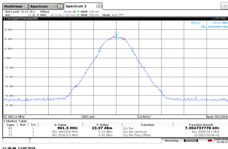
Figure 7.3.2-7: 901.5 MHz – 8FSK (Half Baud) Mode
