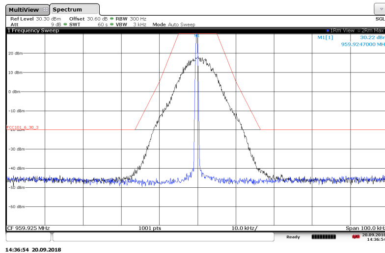
Figure 7.2.2-50: 959.925 MHz – 25 kHz Channel Spacing – m4Pass 20k Mode
