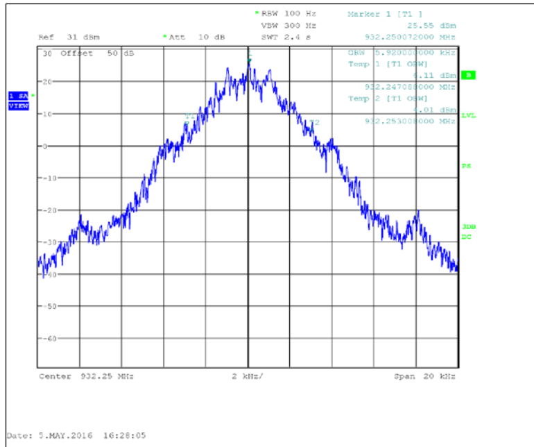
Figure 7.2.3-35: 932.25 MHz — C&amp;I
