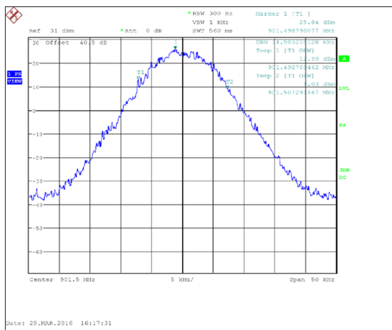
Figure 7.2.3-6: 901.5 MHz – 8SFSK
