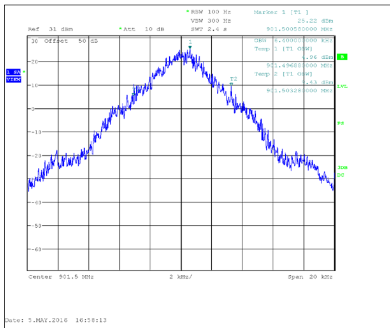
Figure 7.2.3-10: 901.5 MHz – Priority
