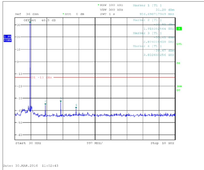
Figure 7.3.2-28: 959.925 MHz – 30 MHz to 10 GHz – m4Pass 20k
