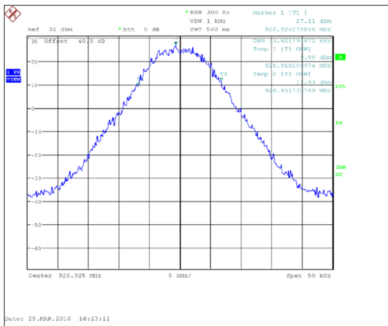
Figure 7.2.3-23: 928.925 MHz — 4SFSK
