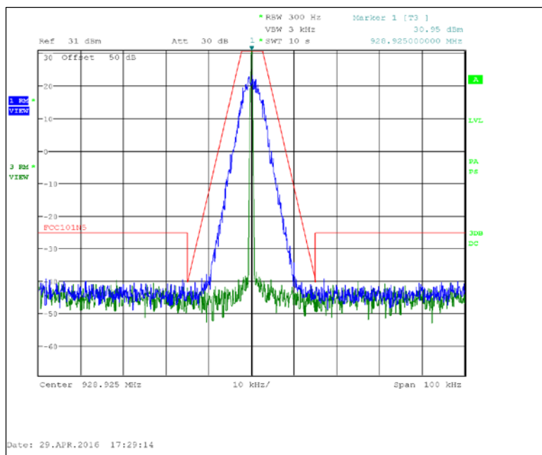
Figure 7.2.2-20: 928.925 MHz – 12.5 kHz Channel Spacing – 8FSK (Half Baud)
