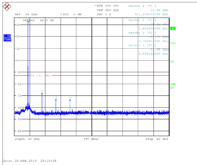
Figure 7.3.2-6: 901.5 MHz – 30 MHz to 10 GHz – 8SFSK
