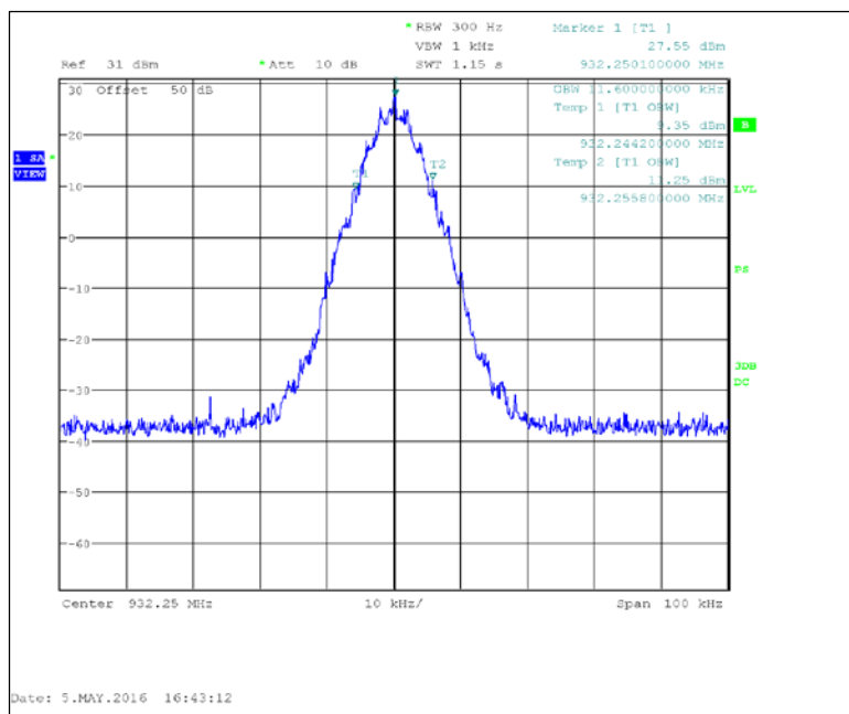
Figure 7.2.3-37: 932.25 MHz — Normal
