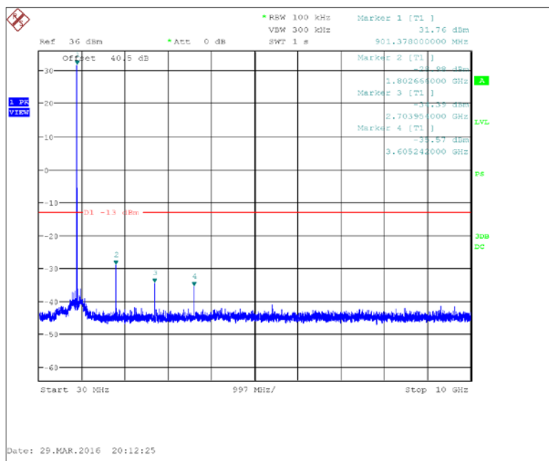
Figure 7.3.2-2: 901.5 MHz – 30 MHz to 10 GHz – 4FSK (Half Baud)
