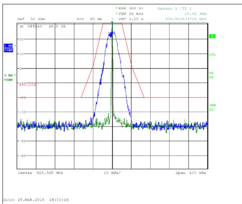
Figure 7.2.2-21: 928.925 MHz – 25 kHz Channel Spacing – 8FSK (Half Baud)
