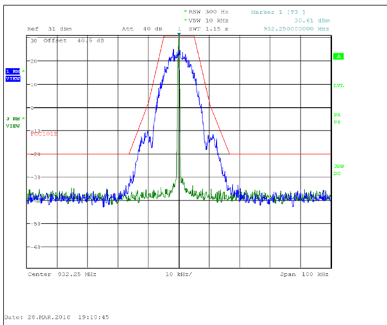
Figure 7.2.2-31: 932.25 MHz – 25 kHz Channel Spacing – 2FSK
