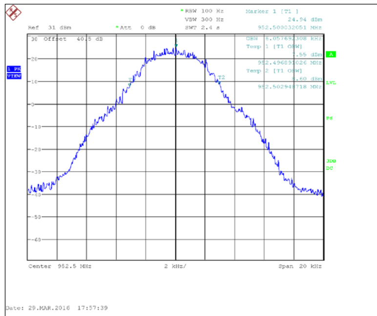
Figure 7.2.3-43: 952.5 MHz – m4Pass 10k Mode
