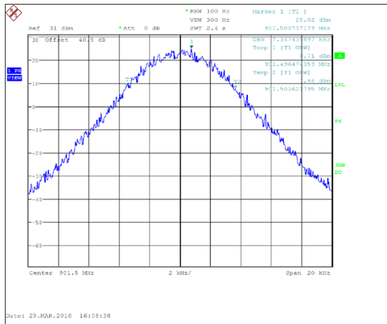
Figure 7.2.3-3: 901.5 MHz – 8SFSK (Half Baud)
