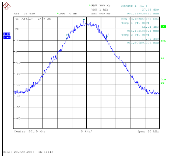
Figure 7.2.3-5: 901.5 MHz – 4SFSK
