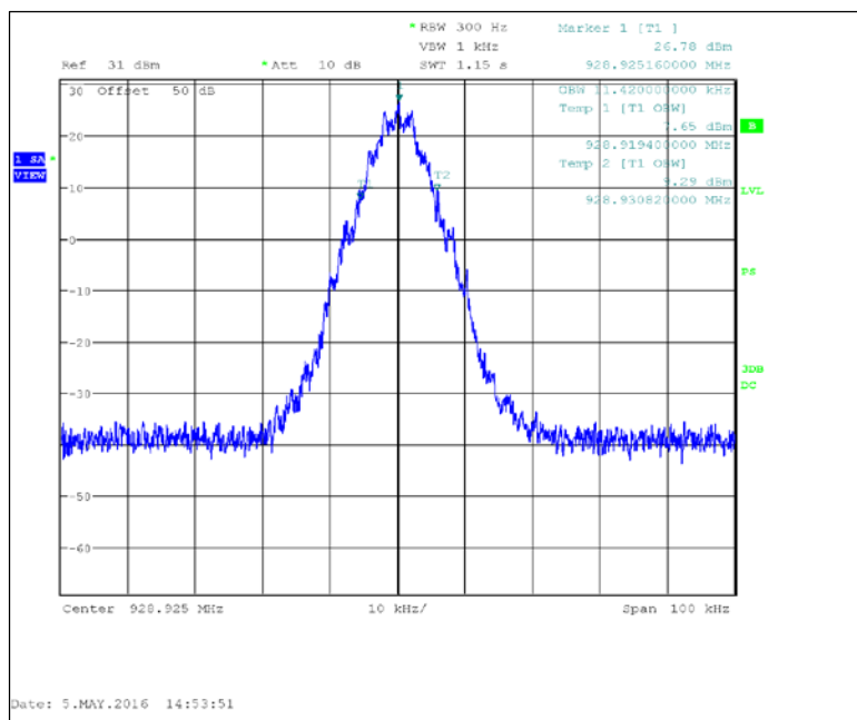
Figure 7.2.3-27: 928.925 MHz — Normal
