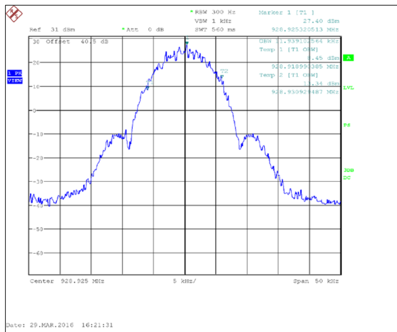
Figure 7.2.3-22: 928.925 MHz — 2FSK
