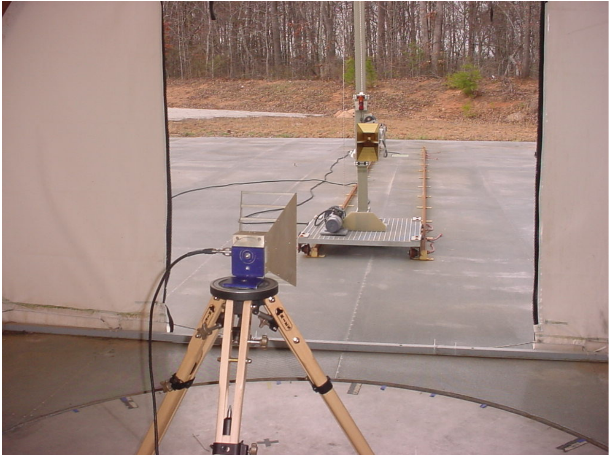
Figure 3: Radiated Emissions - Substitution
