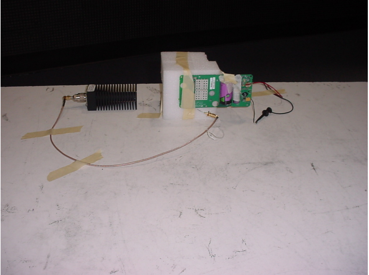
Figure 5: Radiated Emissions - Intentional : 2200-1218-01 Front
