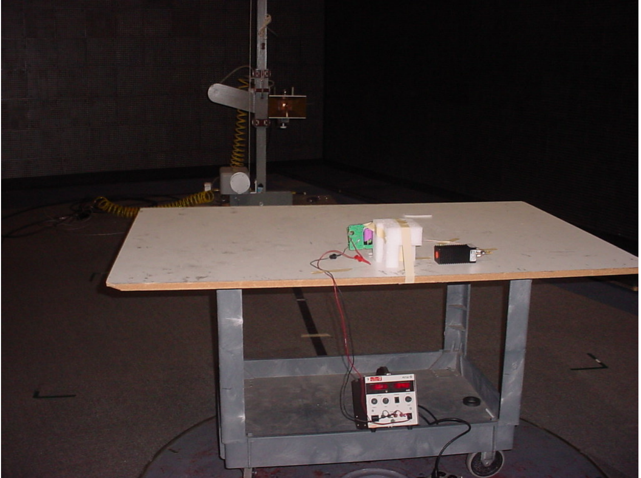
Figure 6: Radiated Emissions - Intentional : 2200-1218-01 Back
