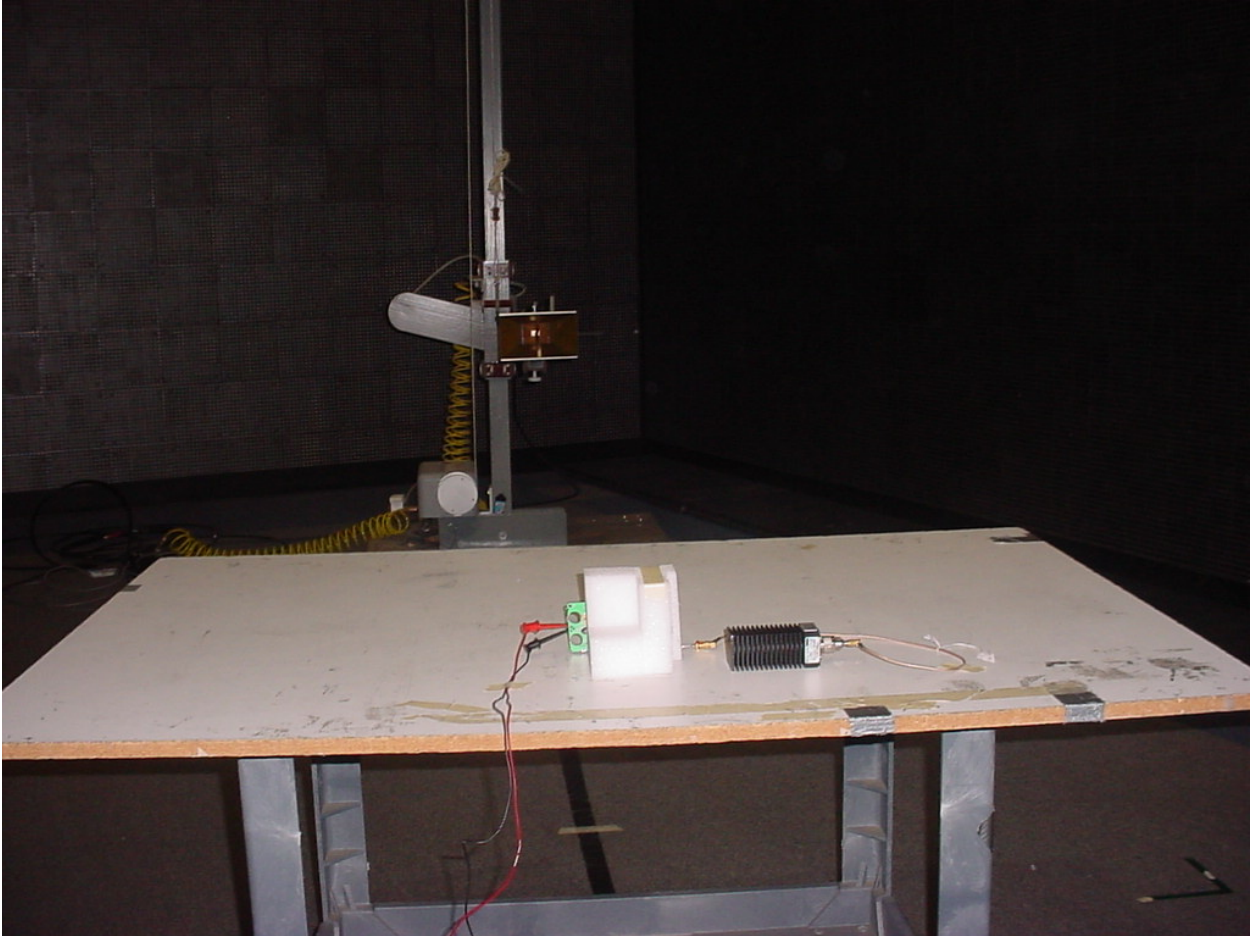
Figure 4: Radiated Emissions - Intentional : 2200-1217-01 Back
