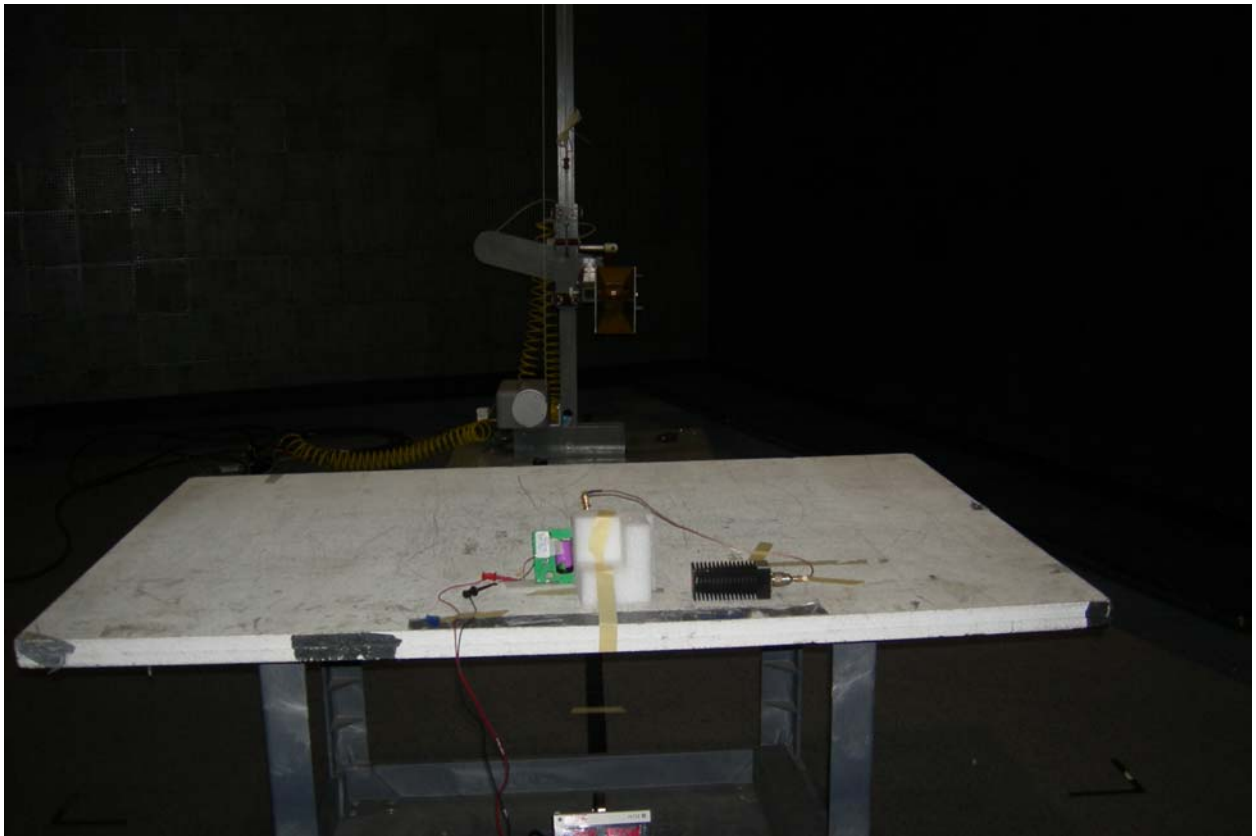
Figure 2: Radiated Emissions - Intentional : 2200-1216-01 Back
