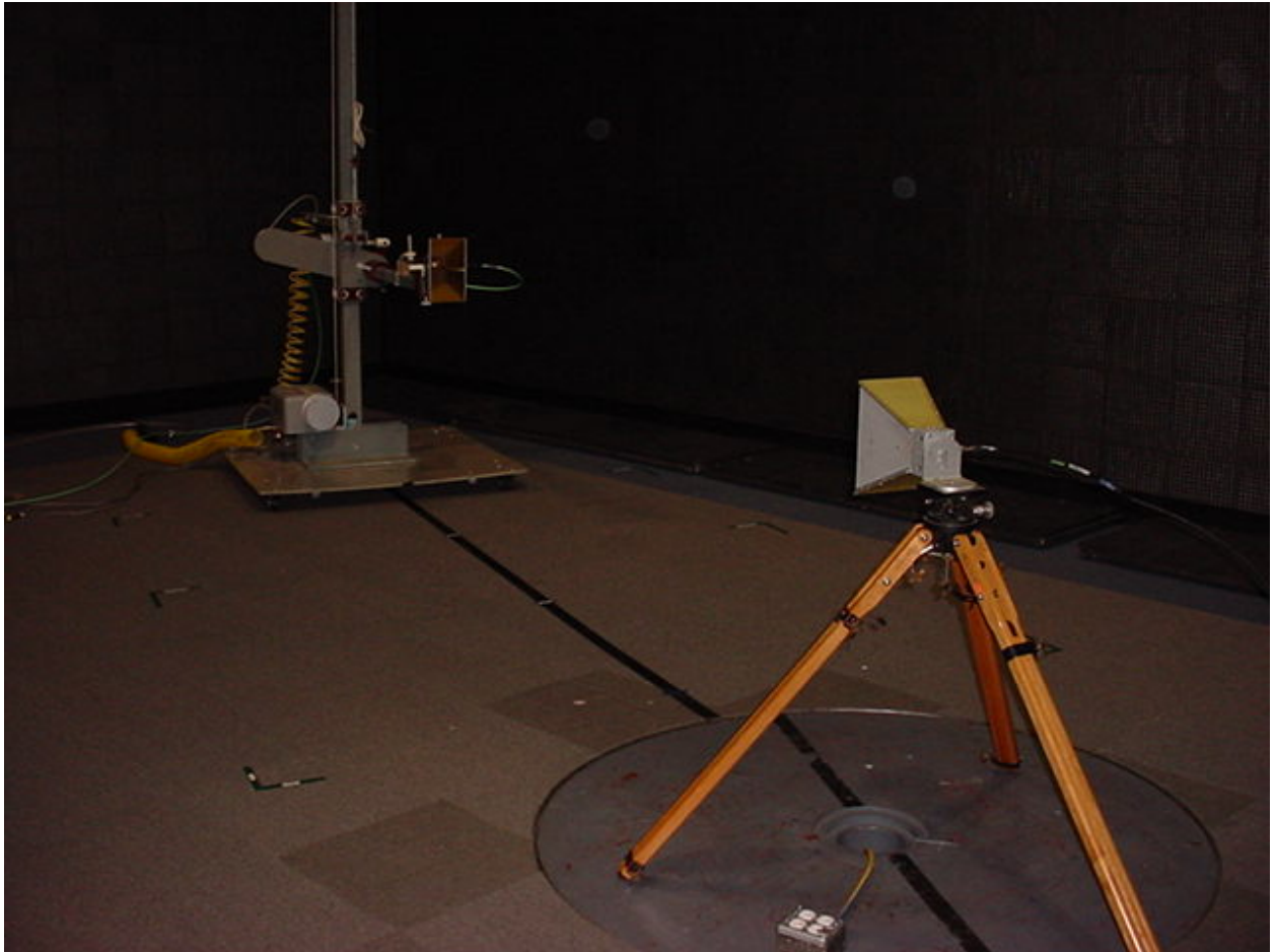
Figure 7: Radiated Emissions - Intentional - Substitution
