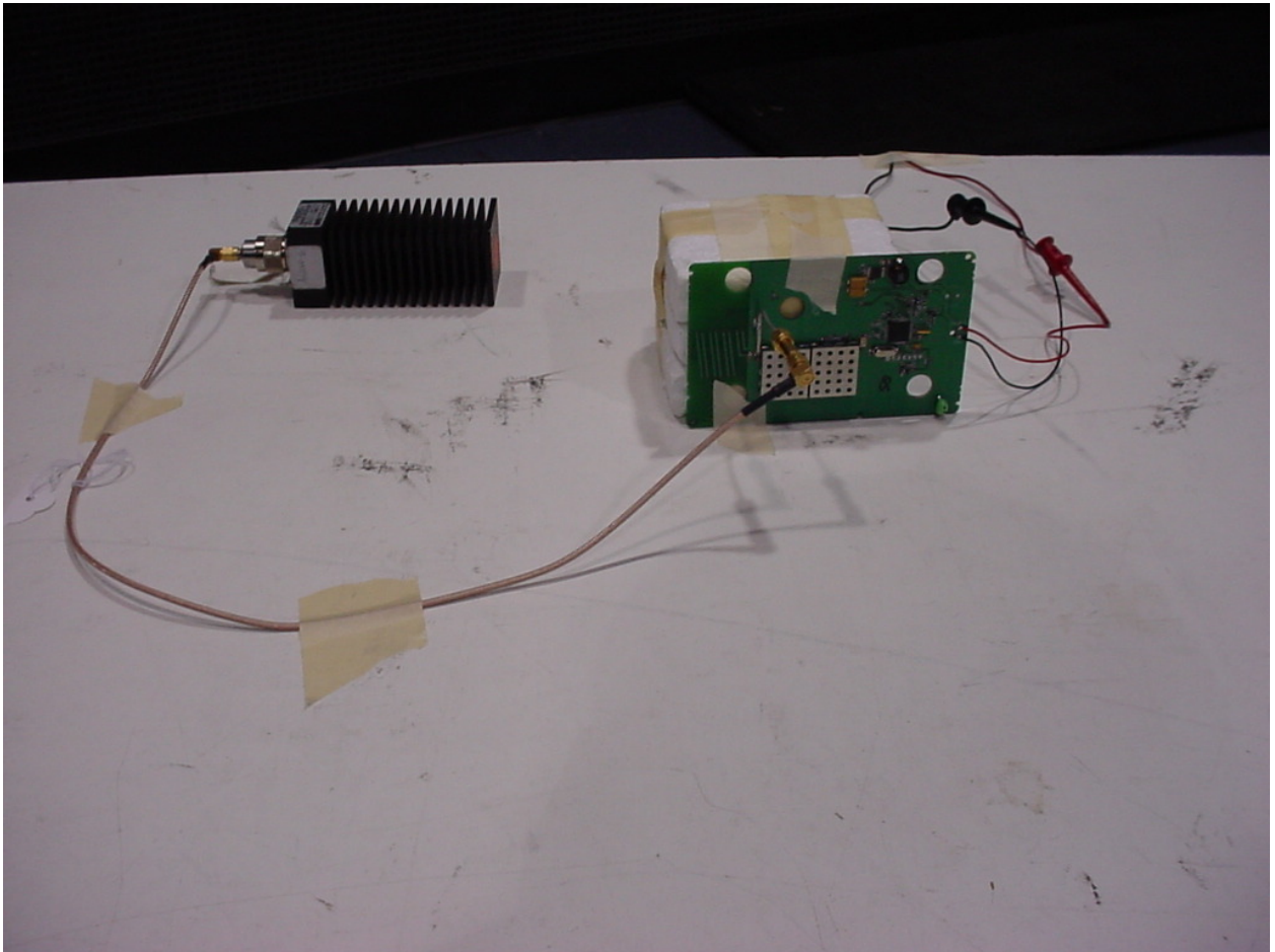
Figure 1: Radiated Emission - Intentional – PCB:0216 Front
