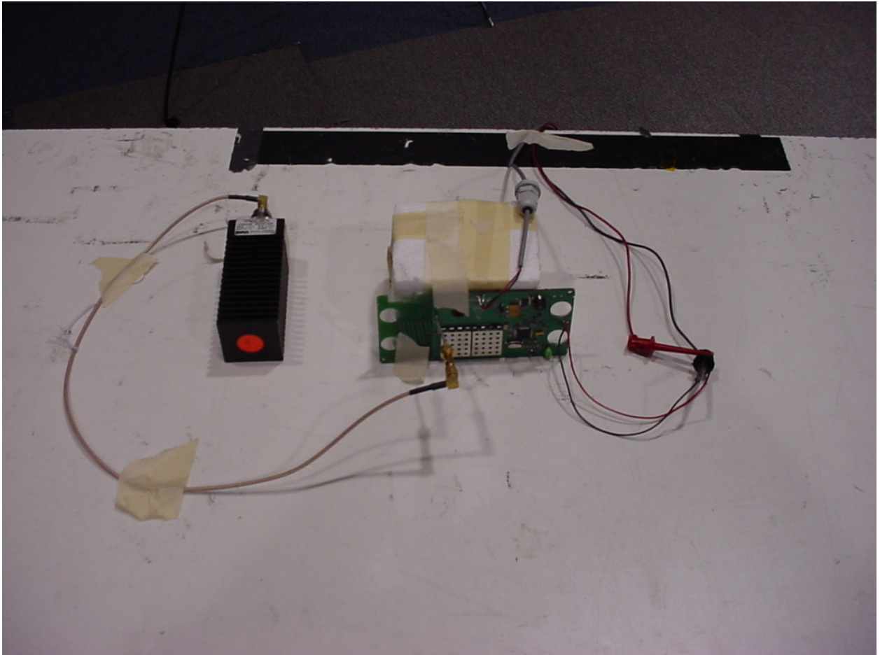
Figure 3: Radiated Emission - Intentional – PCB:0217 Front
