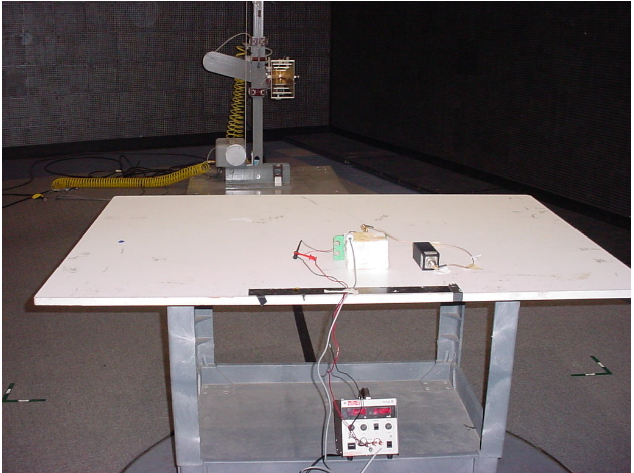
Figure 4: Radiated Emission - Intentional – PCB:0217 Back
