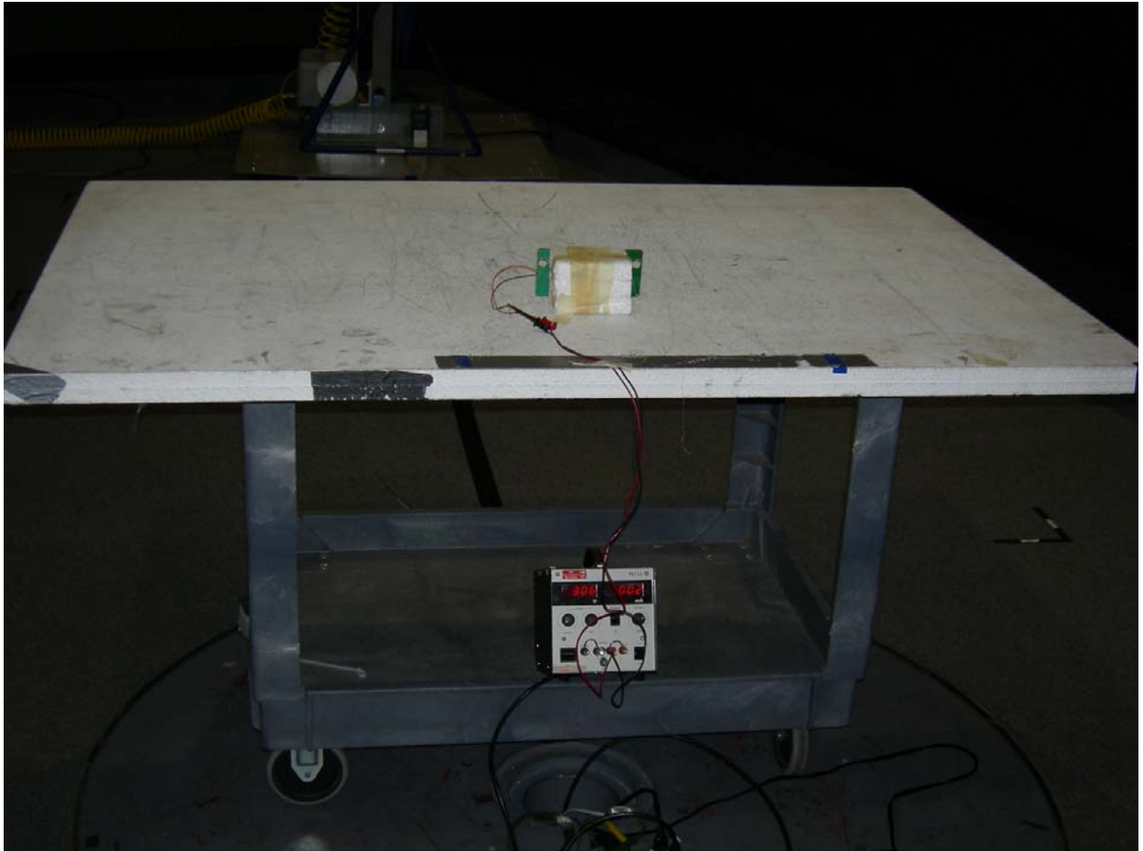
Figure 9: Radiated Emission – Unintentional Back
