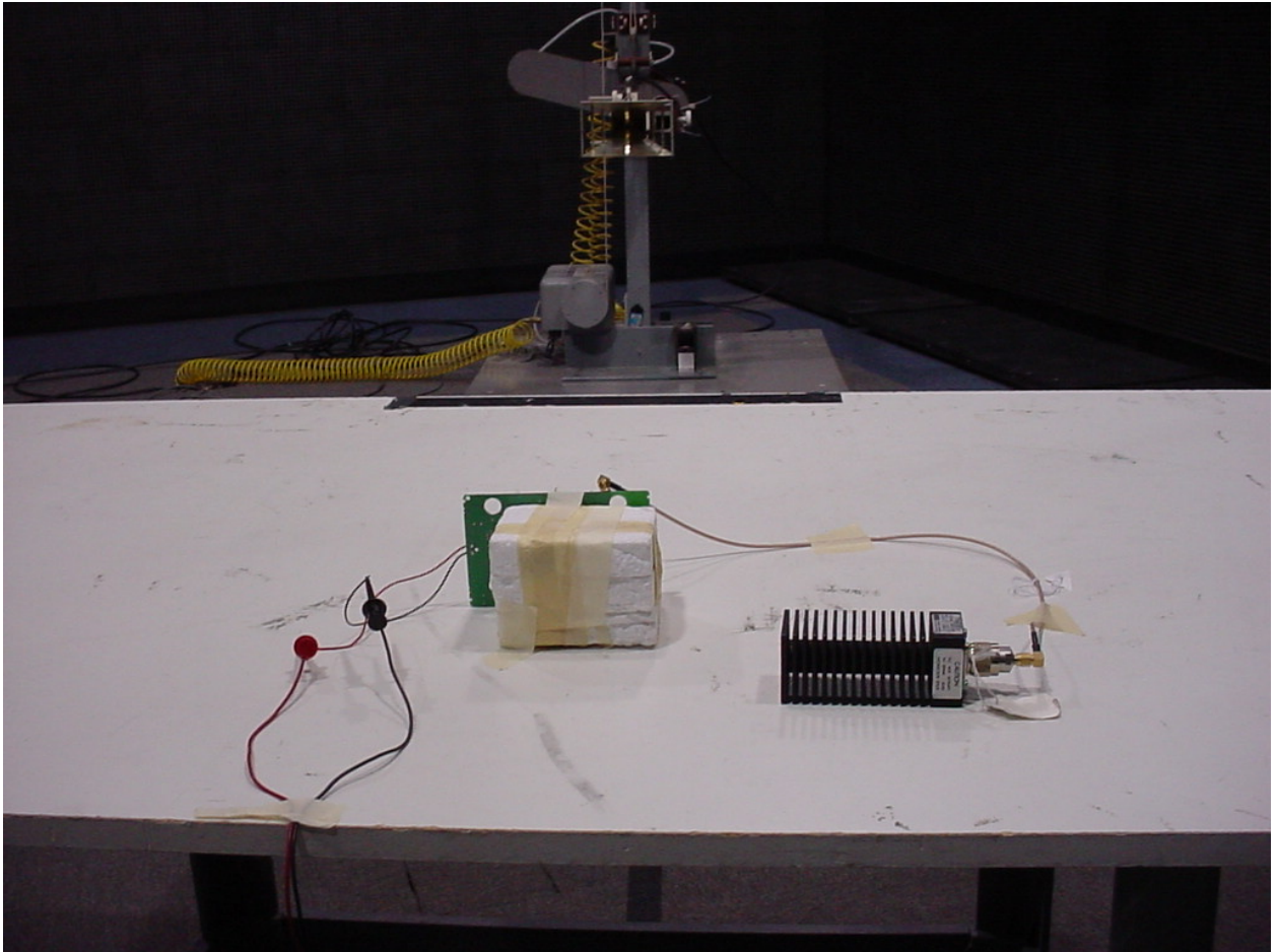
Figure 2: Radiated Emission - Intentional – PCB:0216 Back
