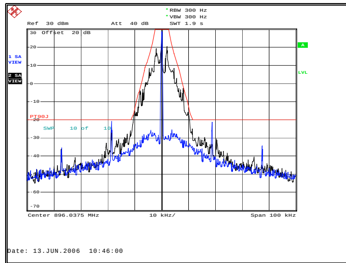
Figure 7.2.3-1: Normal Mode – 896.0375 MHz
