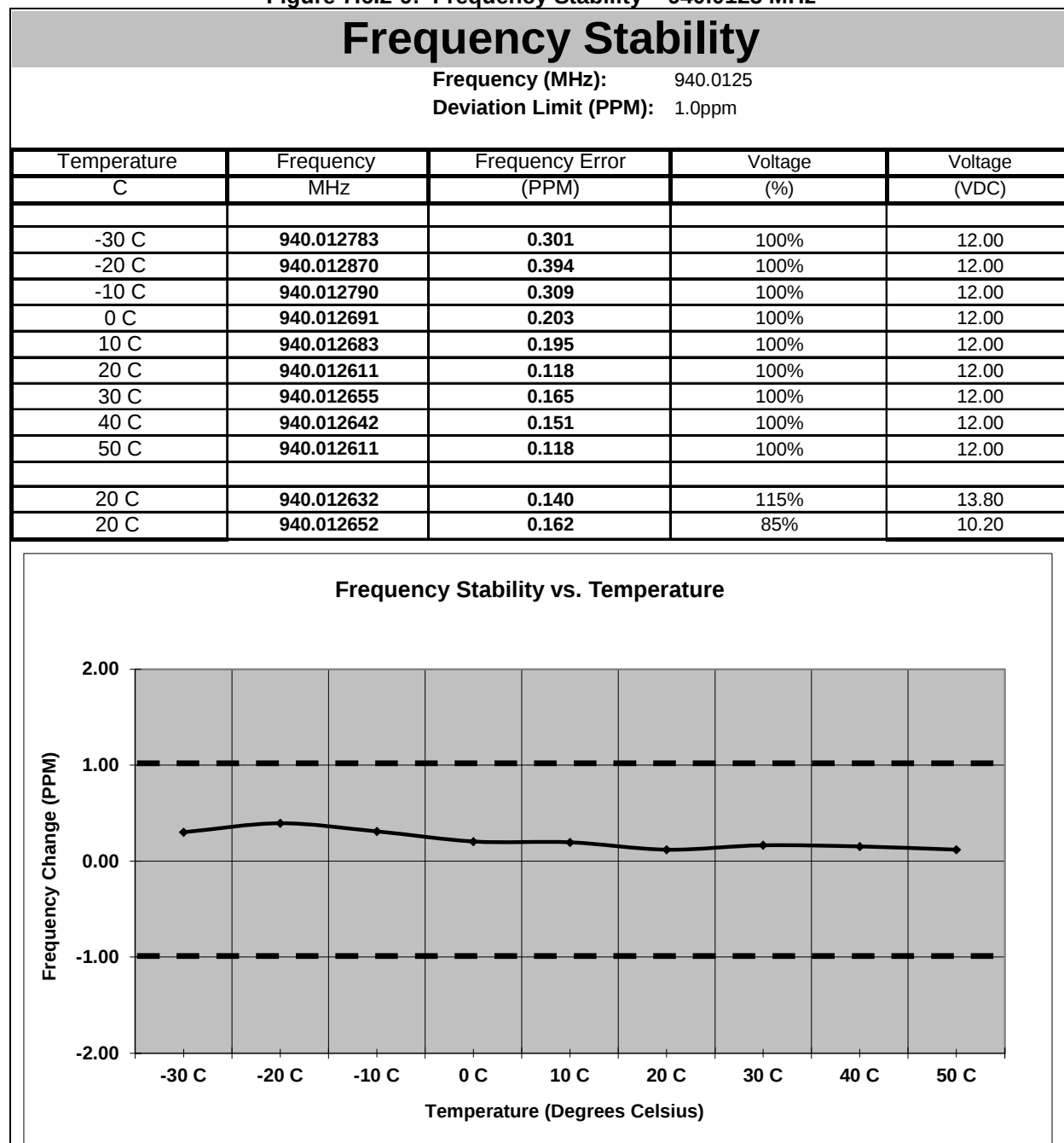
Figure 7.6.2-9: Frequency Stability – 940.0125 MHz
