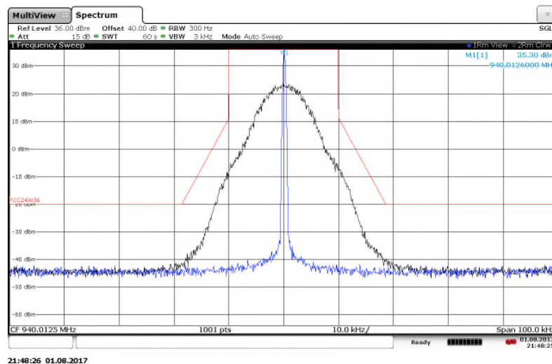
Figure 7.2.2-5: 940.0125 MHz – 25 kHz Channel Spacing – m4pass 20k Mode
