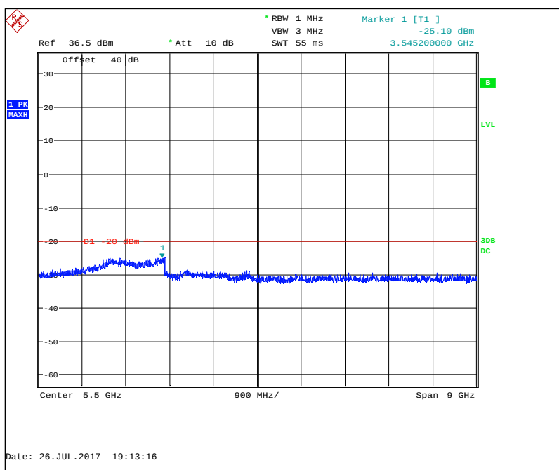
Figure 7.4.2-12: 960 MHz – 1GHz to 10GHz – ERT Tone
