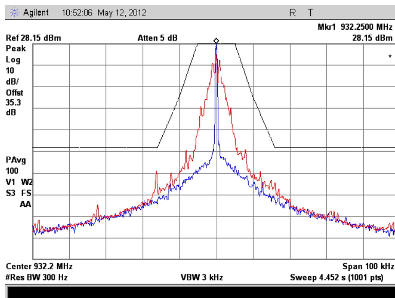
Figure 7.2.2-17: 932.25 MHz –C&amp;I Mode
