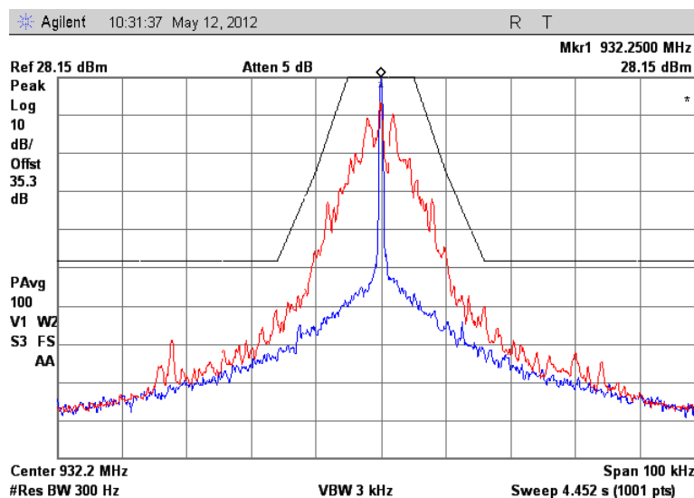
Figure 7.2.2-19: 932.25 MHz –Normal Mode
