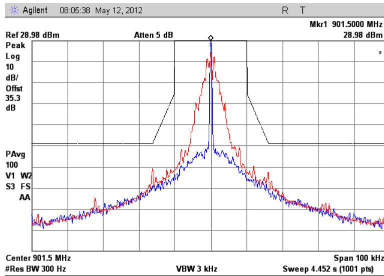
Figure 7.2.2-3: 901.5 MHz – 25 kHz Channel Spacing – C&amp;I Mode
