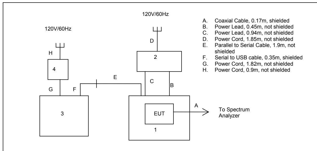
Figure 6-2: EUT Test Setup – RF Conducted Emissions
