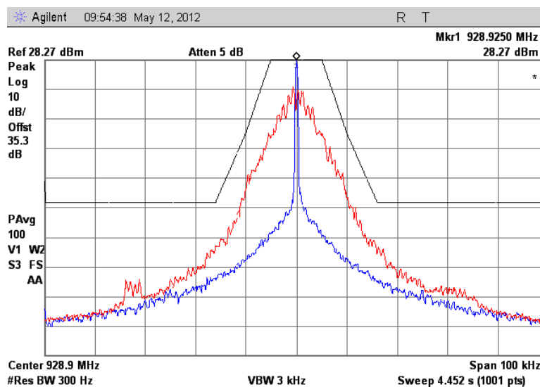
Figure 7.2.2-16: 928.925 MHz — Double Density Mode
