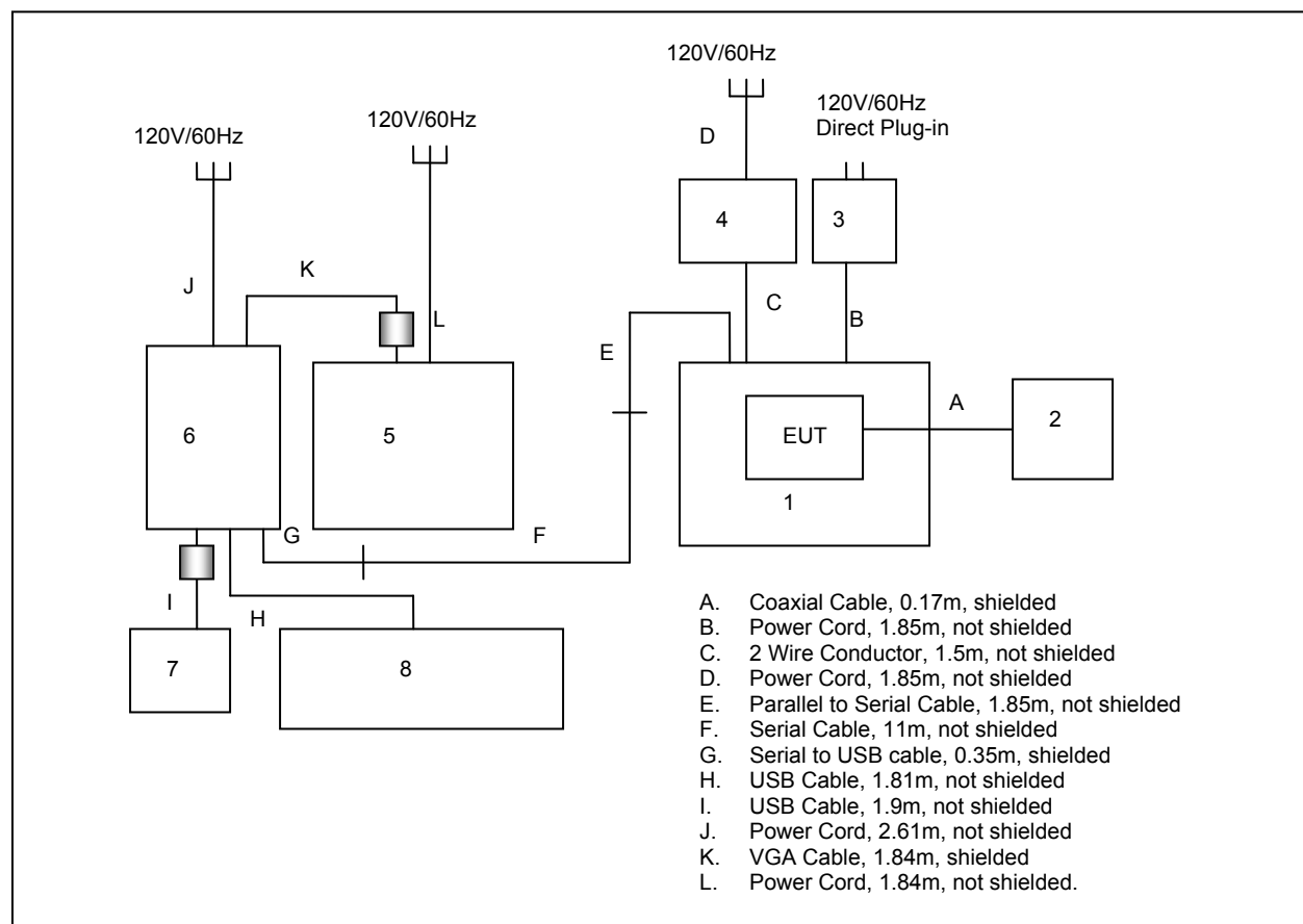
Figure 6-1: EUT Test Setup – Radiated Emissions
